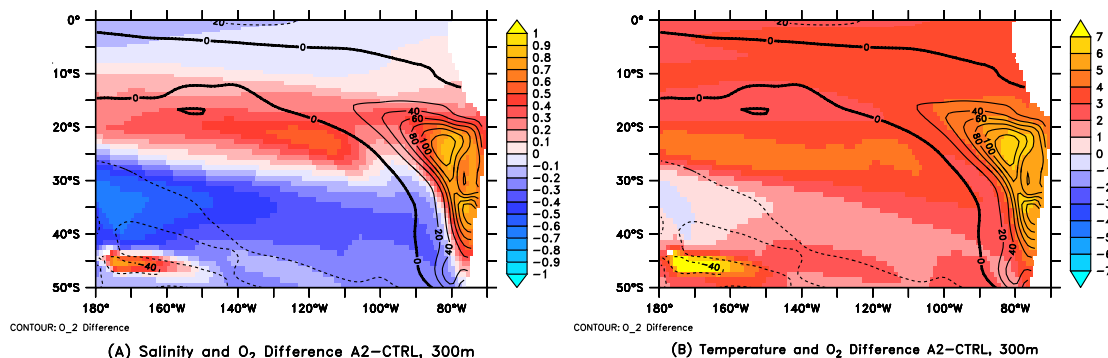
Fig. 2. (A) Change in salinity (A2-CTRL) at 300m in SE Pacific compared with change in oxygen. (B) Same as (A) but for temperature.
