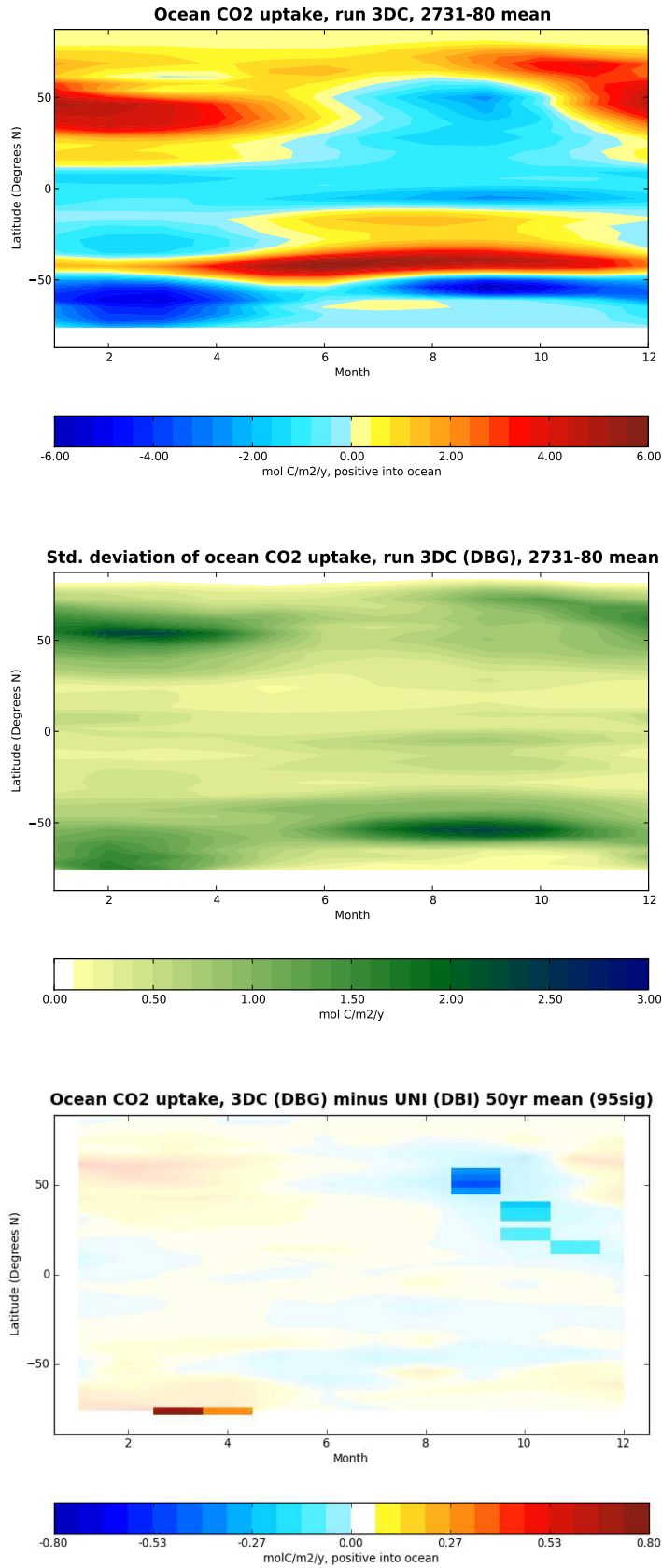
Figure 2: Hovmueller diagrams of 50-year mean zonally averaged: CO 2 uptake by ocean, F ( upper ); interannual standard deviation of F ( middle ), and; difference, \Delta F , between the 3DC and UNI control runs ( lower ). In the lower panel, areas where \Delta F is statistically significant at the 95% level, according to Student's t -test, are overlaid in brighter colours. Each quantity has units of molC m -2 y -1 .
