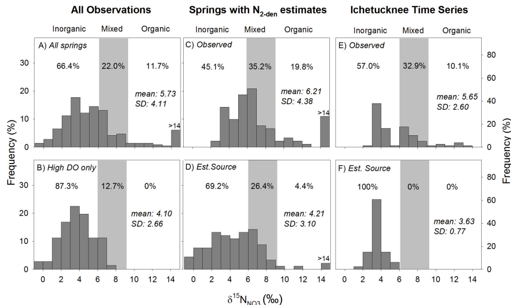
Fig. 9. Implications of fractionation by denitrification for inference of N sources to Florida springs. The distribution of \delta^{15}\text{N}_{\text{NO}_3} across all observations ( A ), among springs sampled for dissolved gases in this study ( C ) and from the Ichetucknee time series ( E ) all suggest meaningful contributions of organic sources (one third to one half of springs). However, \delta^{15}\text{N}_{\text{NO}_3} values in high DO springs ( B ) and source \delta^{15}\text{N}_{\text{NO}_3} as back-calculated from isotopic enrichment factor and denitrification progression ( D , F ) suggest inorganic fertilizers and soil N (from mineralized OM) as the predominant source in the overwhelming majority of springs.
