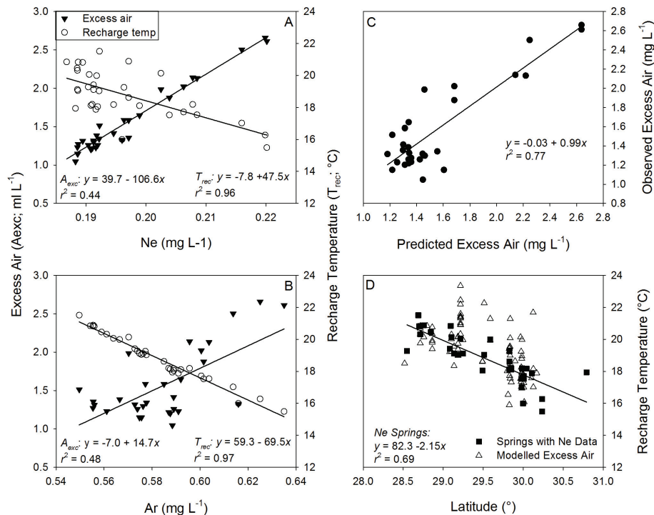
Fig. 2. Geochemical indicators ( A , B ) and springshed predictors ( C , D ) of excess air ( A_{exc} ) and recharge temperature ( T_{rec} ) in Florida springs. ( A ) Ne concentrations are the overwhelming determinant of A_{exc} estimates, and only weakly correlated with T_{rec} ; ( B ) Ar concentrations had relatively small influence on A_{exc} estimates, but a high degree of influence over estimates of T_{rec} . These relationships permit statistical determination of excess air and robust estimation of recharge temperature for springs without Ne measurements. ( C ) A_{exc} across springs was best predicted by the combination of aquifer vulnerability ( V_{aq} ) and spring size as measured by mean historic discharge ( Q_{por} ). ( D ) T_{rec} decreased with increasing latitude, a relationship that is clearer among springs for which Ne data allowed simultaneous direct estimation of A_{exc} .
