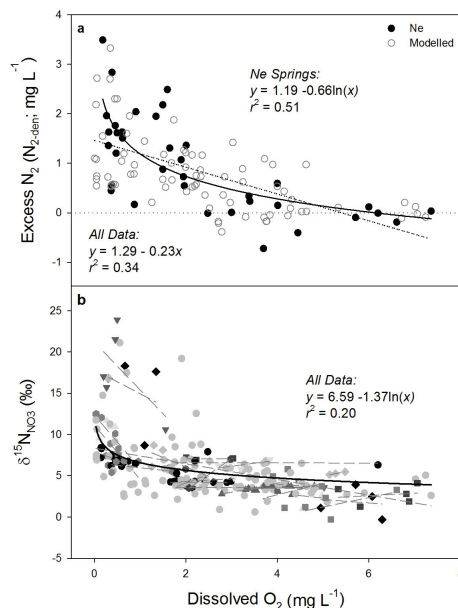
Fig. 4. Dissolved oxygen as a predictor of (a) excess N_2 and (b) \delta^{15}N_{NO_3} in Florida springs. In (a) , closed symbols indicate measurements of denitrification-derived N_2 ( [N_{2,den}] ) based on direct estimation of excess air and recharge temperature via Ne and Ar; best fit for Ne springs is given by the solid line. Open symbols in (a) indicate [N_{2,den}] measurements based on modeled excess air and estimation of recharge temperature from Ar; best fit for all [N_{2,den}] data are shown by the dashed line. In (b) , open symbols indicate data from springs with 3 or fewer observations; closed symbols indicate data from springs with 4 or more observations. Lines in (b) are best-fit linear regressions for individual springs with four or more observations of O_2 and \delta^{15}N_{NO_3} . Springs with high O_2 exhibit little variation in \delta^{15}N_{NO_3} , but low O_2 springs exhibit higher variability in \delta^{15}N_{NO_3} that is linked to variation in oxygen concentrations. Best-fit parameters for individual springs and their relationship to mean dissolved O_2 is shown in Fig. 7.
