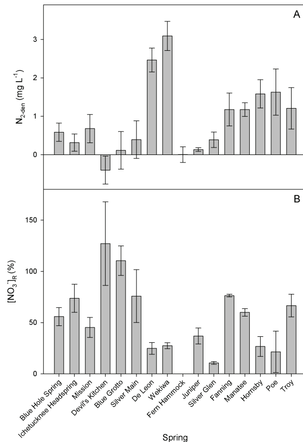
Fig. 5. Variation in the magnitude of denitrification ( [N_{2\text{-den}}] ; panel A ) and residual nitrate pools ( [NO_3^-]_R ; panel B ) within and among springs of the Upper Floridan Aquifer. Variation among springs accounts for more than 90% of total variation in [N_{2\text{-den}}] . Full results of analysis of variance are given in Table 3. Data shown are from all springs with 3 or more estimates of [N_{2\text{-den}}] .
