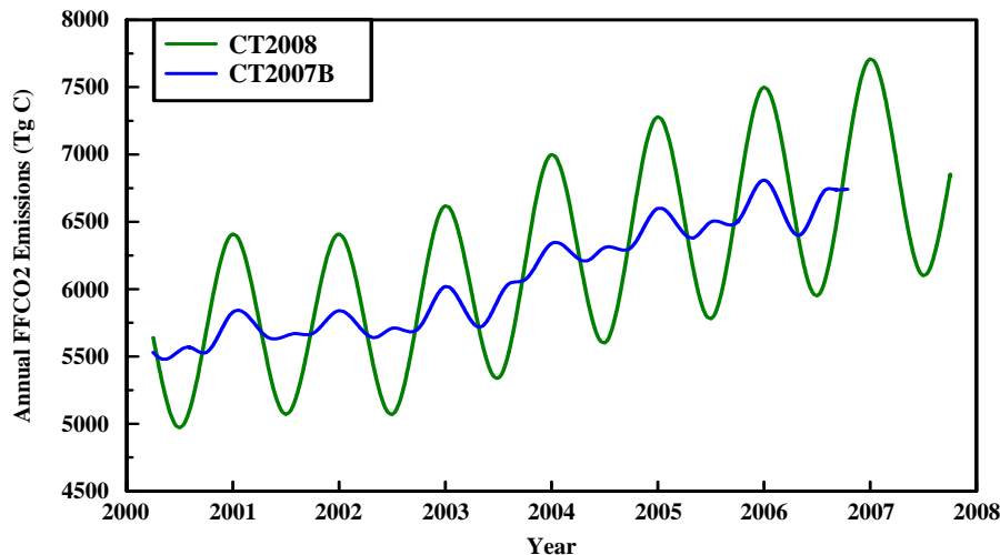
Fig. 6b. Comparison of FFCO 2 emissions from two CT simulations for the CT Northern Land region (between 30°N and 60°N). The first CT release, CT2007B, includes seasonality for North America only (the remainder of the globe used a smooth curve without seasonality). The latter CT release, CT2008, includes seasonality for all land masses. The two curves differ only in the seasonality imposed on the annual totals (see manuscript text for details on the seasonality imposed). The imposition of seasonality to the annual fluxes preserved the exact same annual totals in both schemes. Data from Jacobson (unpublished data).
