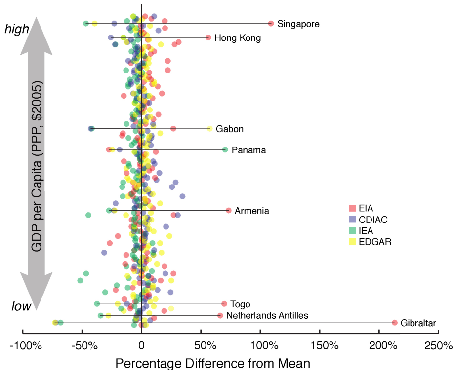
Fig. 2. Differences in total emissions reported by CDIAC, IEA EIA, and EDGAR for 133 nations in 2007. The nations are spread along the y-axis according to their rank-order of GDP per capita (GDP data from the World Bank). Points near zero on the x-axis reflect small differences among the total emissions reported. Outliers reflect larger differences related to the disparate methodologies underlying reported emissions, for instance whether or not emissions from international bunker fuels and calcining of limestone are included.
