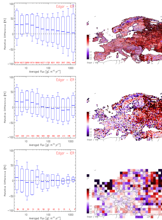
Fig. 7b. Comparison between EDGAR and IER fossil fuel emissions ( \text{gC m}^{-2} \text{yr}^{-1} ) at various spatial resolutions (top to bottom: 1/12, 1/2, and 2 degrees). The right column shows the ratio of EDGAR 4.1 to IER emissions (log scale). The left column shows the binned relative difference (a - b)/(a + b) where a is the EDGAR estimate and b is the IER estimate. The thick horizontal line is the mean, the box indicates \pm one standard deviation, and the whiskers indicate the 10% and 90% percentiles. Perfect agreement would have the mean and standard deviation equal to zero.
