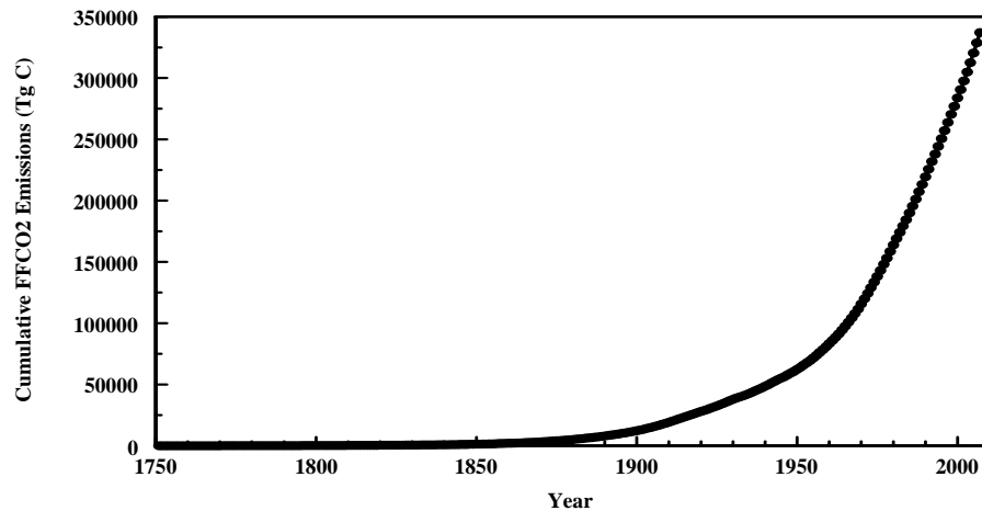
Fig. 3c. Cumulative FFCO 2 emissions from the year 1751 to 2007. This figure was created from summing the data in Fig. 3a. Data from Boden et al. (2010).
