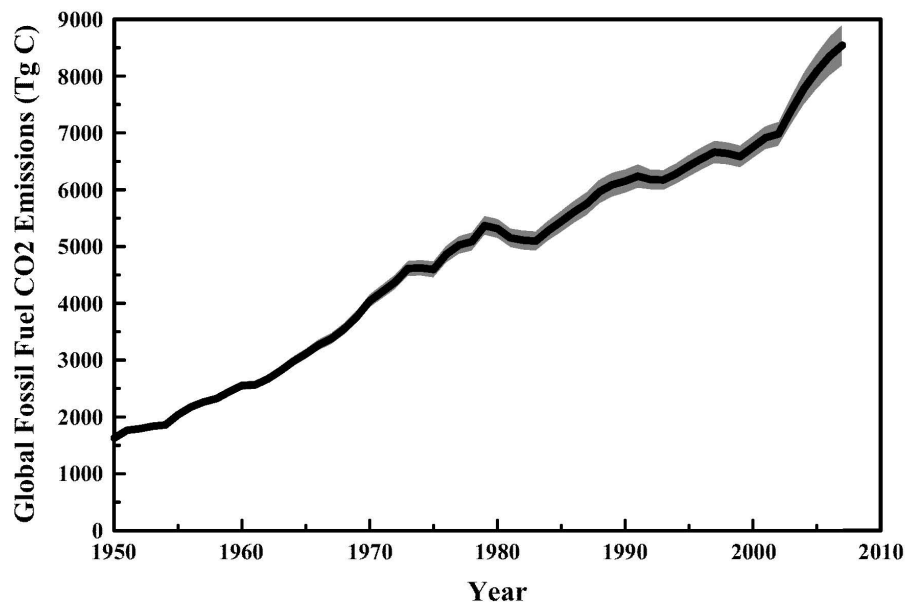
Fig. 7a. Annual FFCO 2 emissions for years 1950 to 2007 with the 95% uncertainty shaded. The shaded area is growing with time because the total magnitude of emissions is growing with time and a growing percentage of emissions are coming from countries with less certainty about their emissions. FFCO 2 data from Boden et al. (2010) and uncertainty estimates from Andres (unpublished data).
