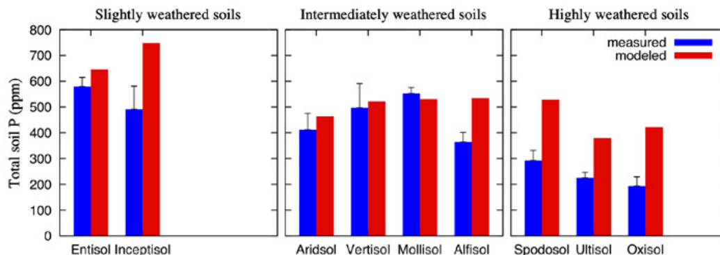
Fig. 4. The comparison of estimated total P with field measurement of total P concentration (mean with one standard error, based on Hedley fractionation data from literature) for soil orders grouped into three weathering categories.
