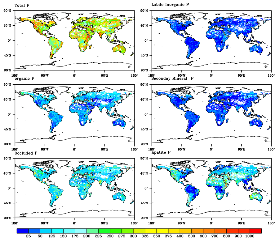
Fig. 3. The distributions of different forms of soil P, each with different accessibility for plant and microbial use (unit: \text{g P m}^{-2} ).
