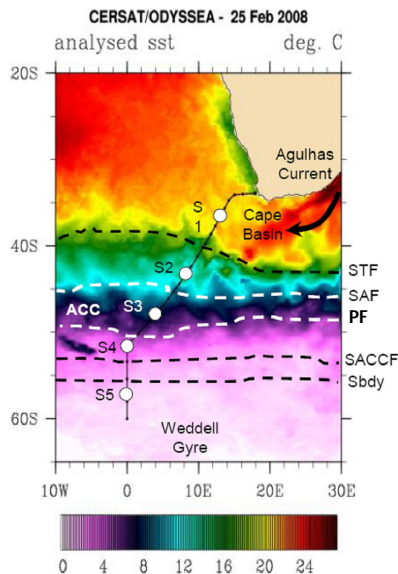
Fig. 1. Left part of panel = BONUS-GoodHope voyage track and super station locations (S1 at 36°31' S; S2 at 42°28' S; S3 at 47°33' S; S4 at 51°52' S; S5 at 57°33' S). The background is Sea Surface Temperature SST (°C) from the CERSAT/ODYSSEA satellite. A SST scale is given at the bottom of the image. The north-south gradient in SST is typical of the region in summer. Approximate location of ACC fronts in summer (STF = Sub-Tropical Front, SAF = Sub-Antarctic Front North, PF = Polar Front, SACCF = South Antarctic Circumpolar Current Front, Sbdy = southern boundary of the ACC) are shown. The area north of the STF is the Sub-Tropical Zone (STZ); the Sub-Antarctic Zone (SAZ) is located between STF and SAF; the Polar Front Zone (PFZ) is located between the SAF and PF; the Antarctic Zone (AZ) is located between the PF and Sbdy, and south of the Sbdy is identified as the northern part of the Weddell Gyre (WG). Right part of panel = Complete salinity S1 PSU (lower panel) and temperature T1 (°C, upper panel) sections during BGH (from BGH cruise report; courtesy from S. Speich ). Station locations are shown.
