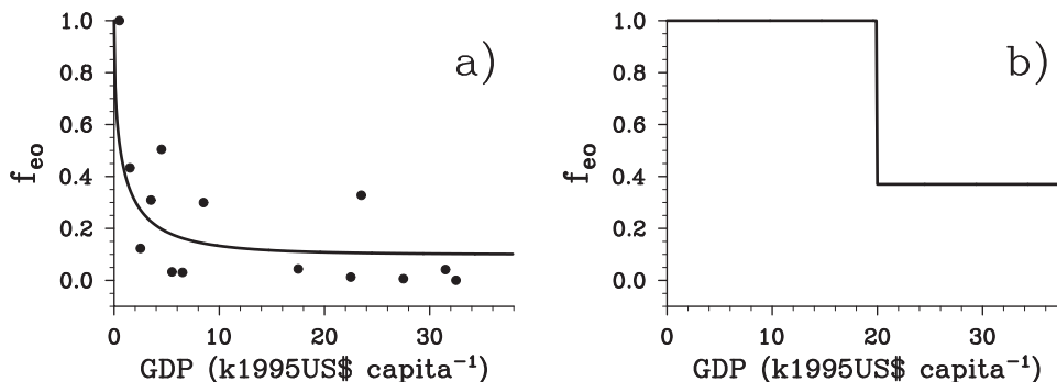
Fig. 5. Effect of economic situation on fire occurrence, f_{eo} , for (a) grass and shrub PFTs and (b) tree PFTs (lines). In shrubs and grasses dominated regions (fractional coverage of shrub and grass PFTs > 50%), 2001–2004 average 0.5^\circ MODIS fire counts are partitioned over 1 k 1995US$capita -1 GDP bins. Black circles in (a) indicate the (normalized) average fire counts in bins with sample size > 5. Goodness of fit are R^2 = 0.73 ( n = 14 ). f_{eo} in (b) reproduces that MODIS fire counts in tree-dominated regions of GDP \geq 20 k 1995US$capita -1 is 0.39 of that in other tree-dominated regions.
