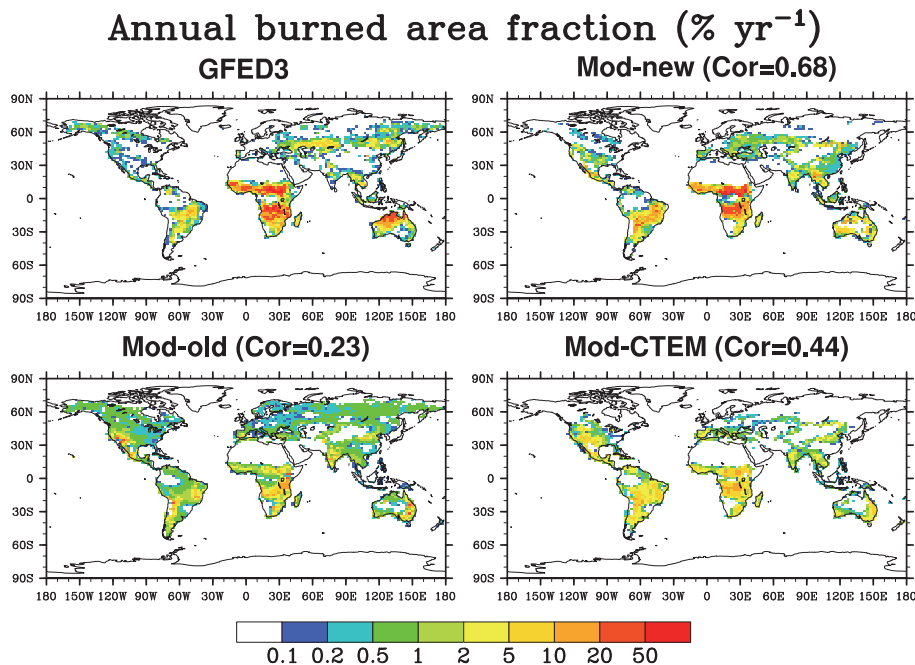
Fig. 9. Spatial distribution of annual burned area fraction averaged over 1997–2004 for GFED3 and CESM1 simulations with different fire parameterizations. The global spatial correlation (Cor) between GFED3 and simulation is also given.
