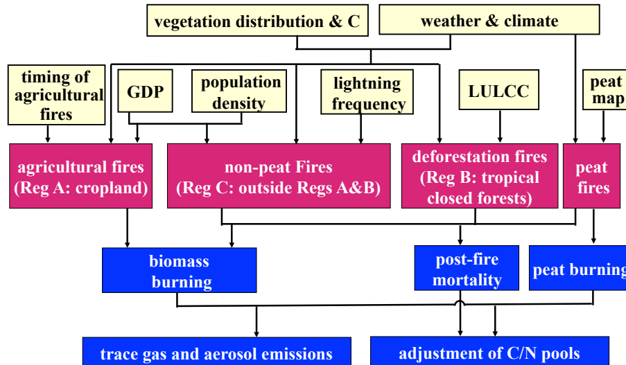
Fig. 2. Structure of new fire parameterization. Fire scheme described in Li et al. (2012) is used in Reg C with modifications by mainly adding the economic influence in the fire occurrence component and the socioeconomic influence in the fire spread component.
