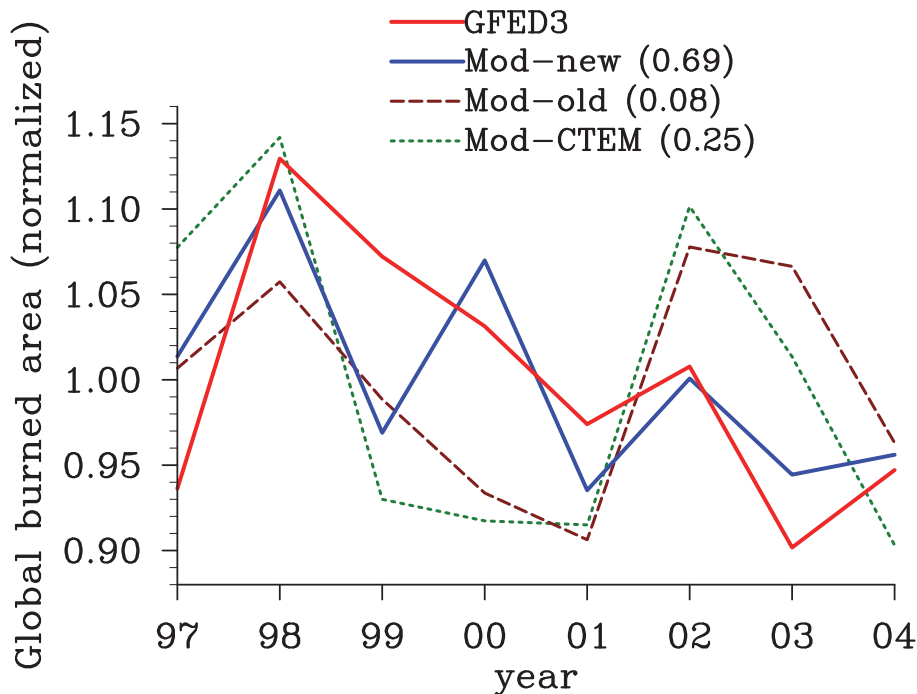
Fig. 13. Annual global burned area normalized by the mean for 1997–2004 from GFED3 and CESM1 simulations with different fire parameterizations. The numbers in brackets denote temporal correlation between GFED3 and simulations.
