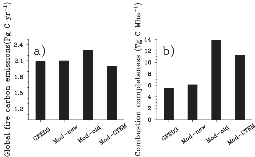
Fig. 14. 1997–2004 average (a) global annual fire carbon emissions and (b) combustion completeness in global post-fire regions.
