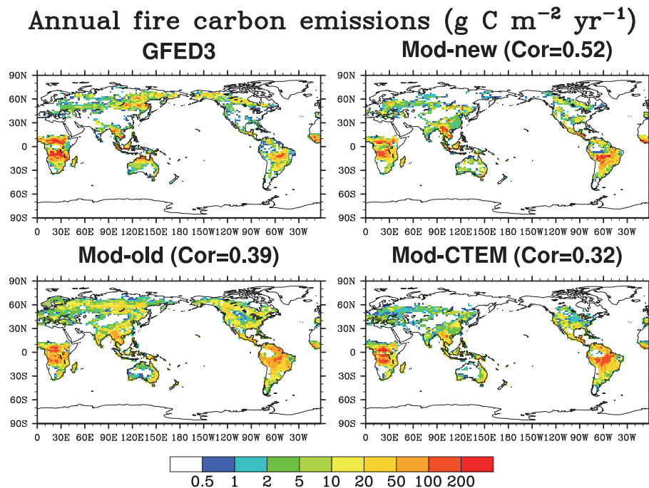
Fig. 16. Same as Fig. 9, but for annual fire carbon emissions.
