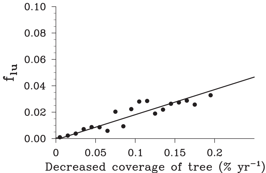
Fig. 4. Effects of decreases of tree coverage on annual burned area, f_{lu} (Line). 0.5^\circ GFED3 burned area fraction in Amazon rainforest (tropical closed forest in 15.25^\circ S– 10.25^\circ N, 30.75^\circ – 90.75^\circ W) are partitioned over 0.01\% \text{ yr}^{-1} deforestation rate bins. Black circles indicate the average burned area fraction in bins with sample size > 5 . Goodness of fit is 0.83 ( n = 19 ).
