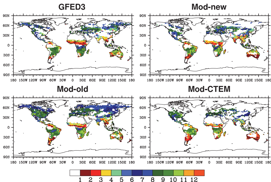
Fig. 11. Same as Fig. 9, but for month of maximum burned area for those areas where burned area fraction > 0.1 %.
