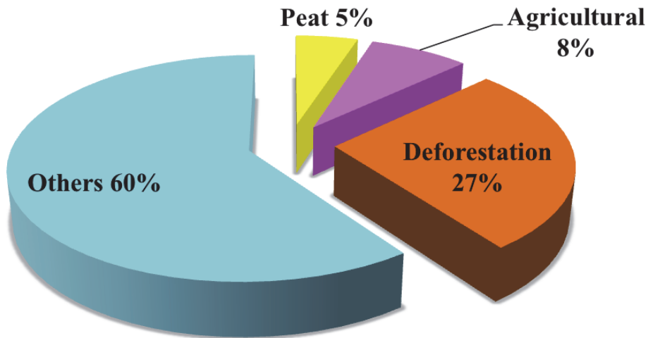
Fig. 15. Contribution of agricultural fires, tropical deforestation and degradation fires, non-peat fires outside cropland and tropical closed forests, and peat fires to 1997–2004 global fire carbon emissions from Mod-new.
