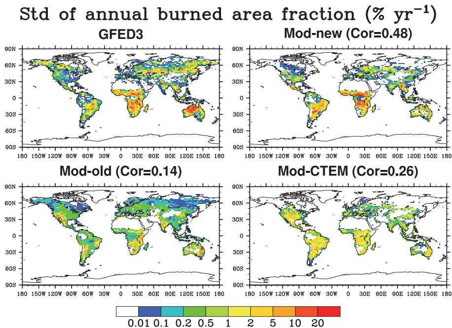
Fig. 12. Same as Fig. 9, but for standard deviation (Std) of annual burned area fraction which is used as a spatially-explicit measure of fire interannual variability.
