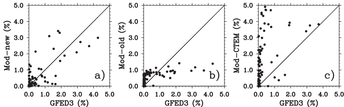
Fig. 10. Comparison of GFED3 and modeled 1997–2004 average annual burned area fraction over Amazon tropical closed forest. The black line depicts the 1 : 1 slope and represents the perfect simulation. Relative mean squared error (MSE divided by the variance of GFED3 annual burned area fraction) is 0.39 for Mod-new, 0.72 for Mod-old and 2.72 for Mod-CTEM.
