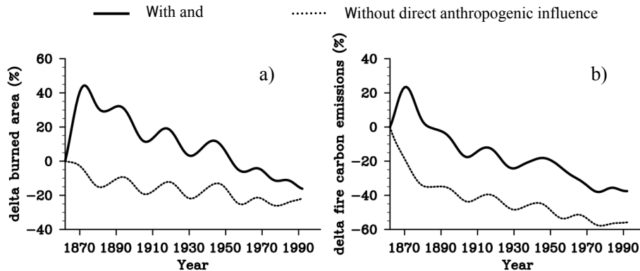
Fig. 18. Historical variation of (a) global burned area and (b) fire carbon emissions in simulations with and without direct anthropogenic influence. 25-yr low-pass filter is used.
