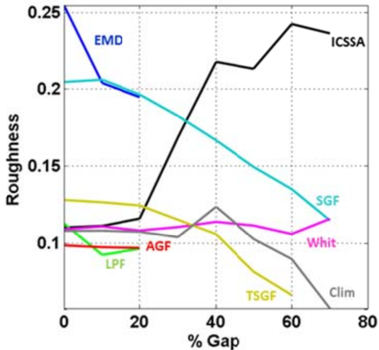
Fig. 8. Roughness of LAI_{rec} as a function of % Gap in LAI_{sim} .
