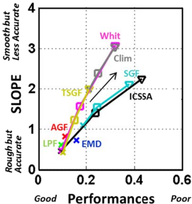
Fig. 11. Performances (distance to the origin) and slopes in the [Roughness, RMSE] feature plane (Fig. 10) associated to each method for 0\% < \% \text{ Gap} < 15\% (X), 25\% < \% \text{ Gap} < 35\% (□) and 35\% < \% \text{ Gap} < 45\% (▽). Note that EMD, LPF and AGF are only displayed for the lowest % Gap class. The black arrow indicates the effect of an increase of the fraction of missing data.
