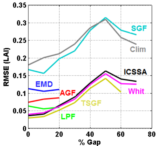
Fig. 6. RMSE as a function of %Gap. The RMSE is computed between LAI_{ref} and the reconstructed LAI_{rec} time series over dates with actual observations in LAI_{sim} . The values were slightly shifted vertically to ease the reading when curves were overlapping.
