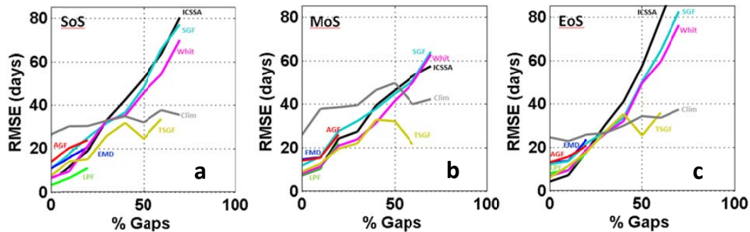
Fig. 9. RMSE relative to the timing (in days) of the start of season (a) , maximum of season (b) and end of season (c) . The RMSE is evaluated between the phenological dates computed with LAI_{ref} and those derived from the reconstructed LAI_{rec} time series using the several methods investigated.
