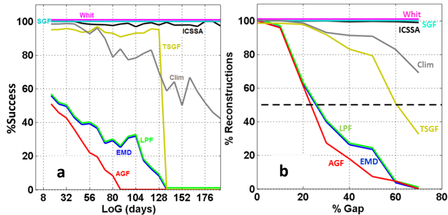
Fig. 5. (a) Fraction of gaps reconstructed (% Success) as a function of the length of the gaps (LoG). (b) Fraction of missing data reconstructed (% Reconstructions) as a function of the % Gap. The horizontal dashed line represents the 50 % threshold of % Reconstructions. The several methods are represented by different colors. Some values were slightly shifted vertically to ease the reading when curves were overlapping.
