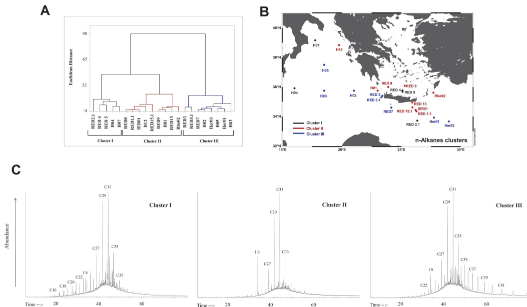
Fig. 5. Hierarchical diagram obtained from cluster analysis of all stations with regard to n -alkanes profile (A) , clustered station sites (B) and characteristic GC-MS chromatographs for each returning cluster (C) . Cluster I: Station H03, Cluster II: Station RED9 and Cluster III: Station Her03. I.S: Internal Standard.
