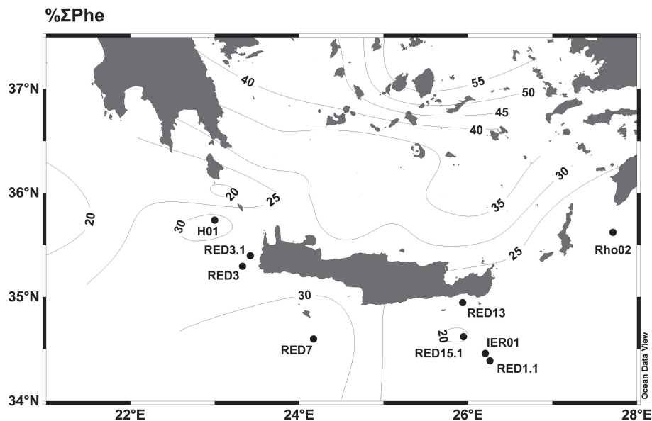
Fig. 8. Spatial distribution of \% \Sigma \text{Phe} in Cretan Sea (southern Aegean Sea) and western Cretan-Antikythera straits surface sediments. Data for Cretan Sea sediments are a combination of data reported in this study and data reported (stations not shown) by Hatzianestis and Sklivagou (2001).
