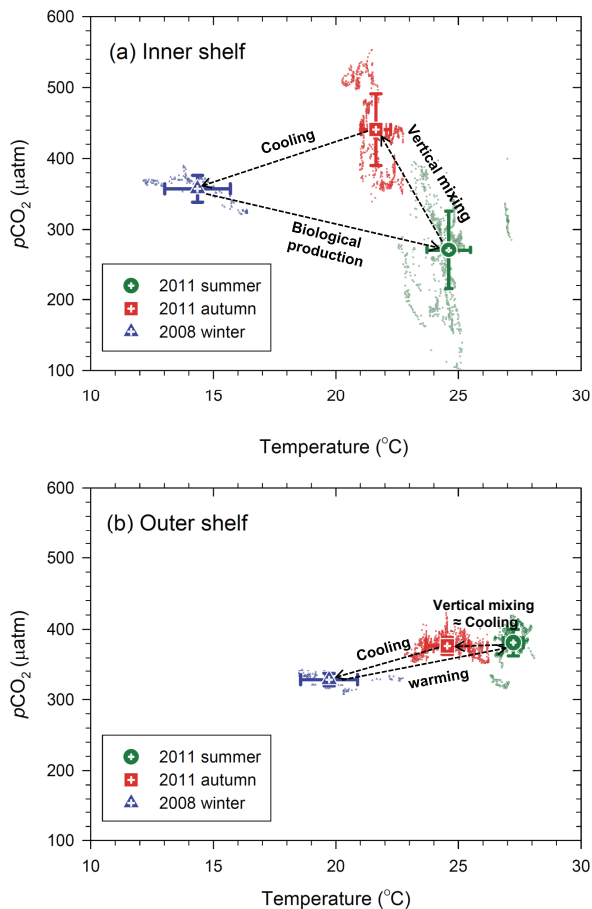
Fig. 5. Plots of p\text{CO}_2^{\text{sw}} vs. temperature for summer 2011, autumn 2011, and winter 2008 data in (a) the inner shelf area and (b) the outer shelf area. The definitions of the inner and outer shelf areas are the same as in Fig. 2.
