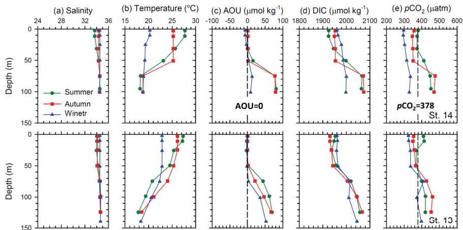
Fig. 4. Depth distributions of (a) salinity, (b) temperature, (c) AOU, (d) DIC, and (e) p\text{CO}_2^{\text{sw}} in summer, autumn, and winter at the stations with modest seasonal variations of p\text{CO}_2^{\text{sw}} (stations 13 and 14 in the outer shelf).
