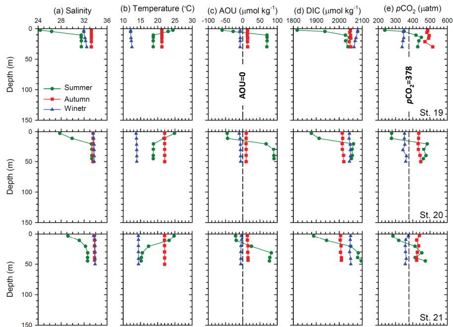
Fig. 3. Depth distributions of (a) salinity, (b) temperature, (c) AOU, (d) DIC and (e) pCO 2 sw in summer, autumn, and winter at the stations with the largest seasonal variation of pCO 2 sw (stations 19, 20, and 21 in the inner shelf near the Changjiang Estuary).
