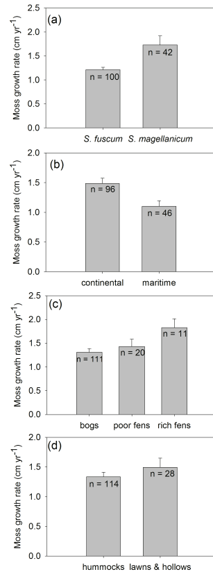
Fig. 2. Sphagnum growth values (mean and standard error) for each species (a) , continentality class (b) , peatland type (c) , and microform (d) .
