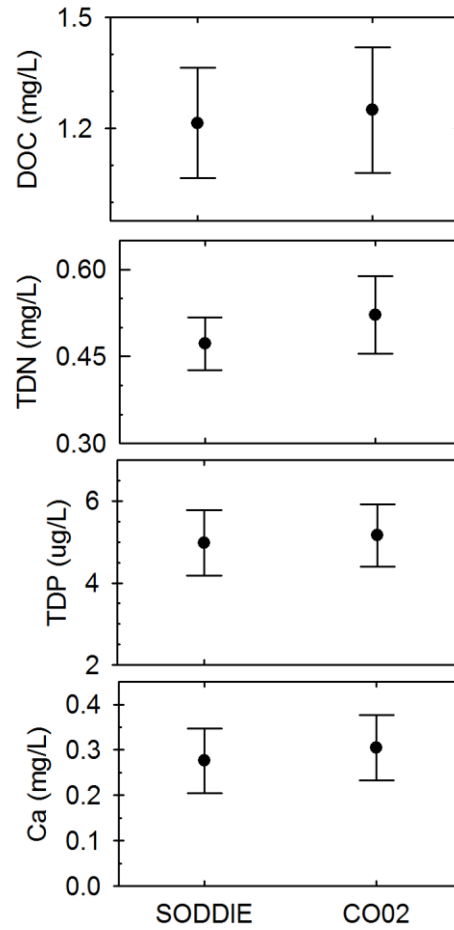
Figure S3. Mean concentrations with 95% confidence intervals for dissolved organic carbon (DOC), total dissolved nitrogen (TDN), total dissolved phosphorus (TDP) and calcium (Ca) from 2002-2010 for Soddie and CO02 NADP collectors. Only samples with precipitation > 500 g were considered. None of the concentration values were significantly different from each other at a level of p \leq 0.01 .
