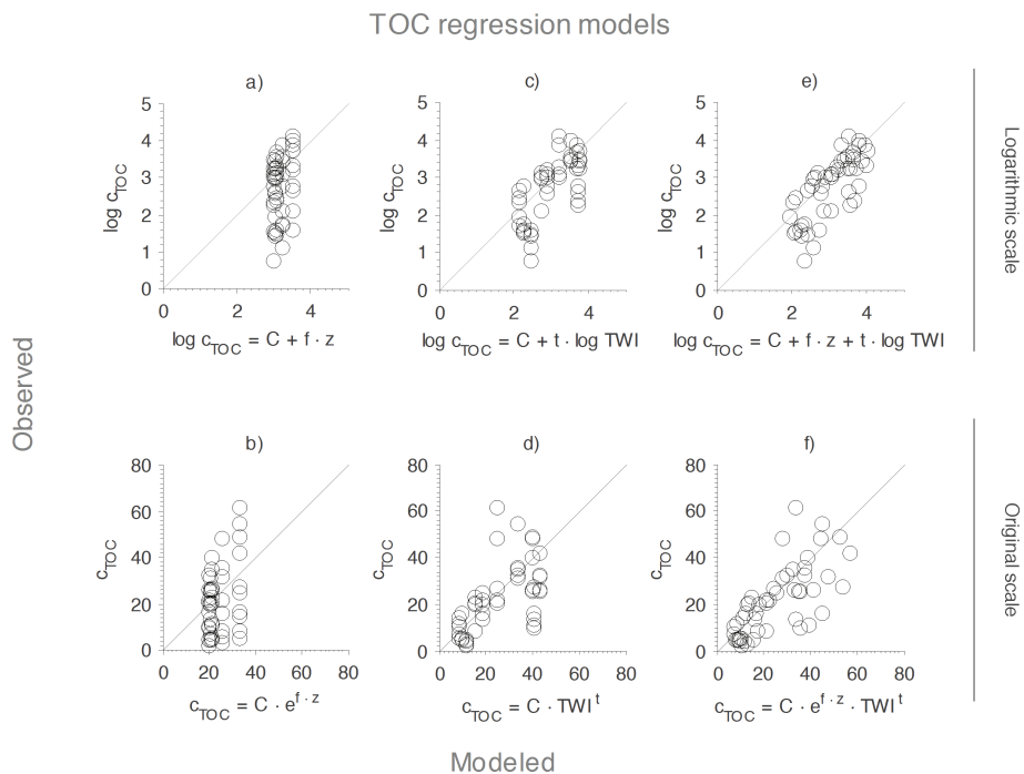
Fig. 7. Modeled versus predicted average TOC concentrations (empty circles) for 10 riparian monitoring sites and 5 different depths (15, 30, 45, 60 and 75 cm below the surface) in the till part of the catchment. In the upper row log-transformed TOC concentrations are shown. Three regression models for TOC were tested using depth (first column), TWI (middle column) as well as using both depth and TWI as predictors (right column).
