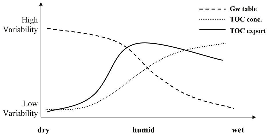
Fig. 8. Temporal variability as function of riparian zone wetness for different quantities (schematic figure).
