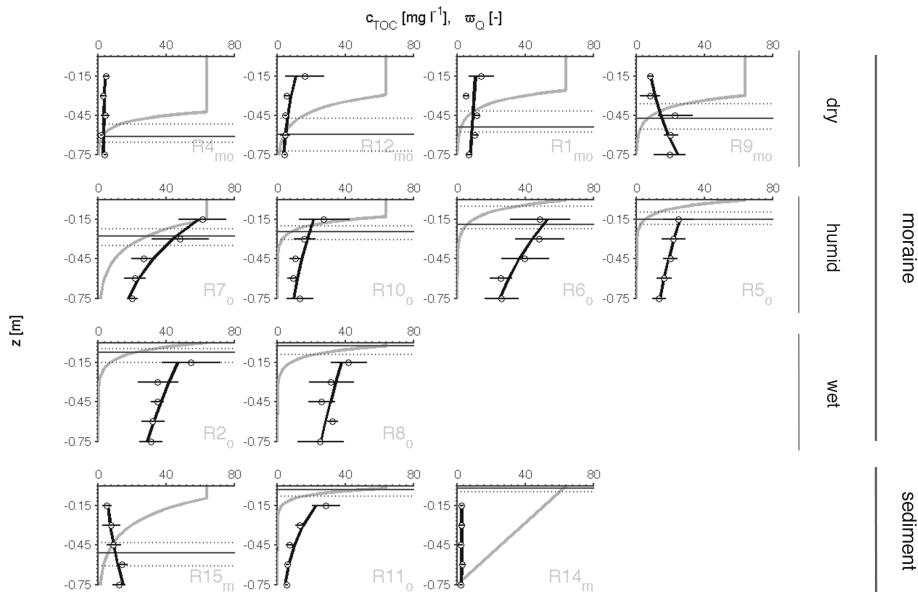
Fig. 3. Average TOC concentrations c_{\text{TOC}} (circles) from 9 sampling occasions (2008–2009), interpolated TOC profiles (black lines), median groundwater position (solid, grey horizontal line) and the (dimensionless) weighting functions \omega obtained from lateral flow profiles (light-grey curves) for all 13 sites. The range of temporal variability of TOC concentrations at different depths is represented by horizontal black lines (average concentration \pm 1 standard deviation) and the range of temporal variability of groundwater positions is indicated by dotted grey horizontal lines (10th and 90th percentile of groundwater positions). Each subplot contains a site label located in the lower right corner. The subscripts next to each site number in the labels indicate mineral (m), mineral-organic (mo) and organic (o) soil profiles. Rows 1 to 3 represent soil plots underlain by till deposits and sorted according to increasingly shallow average groundwater positions (dry, humid and wet locations in the 1st, 2nd and 3rd row respectively). The lower 4th row contains sites underlain by sediment deposits.
