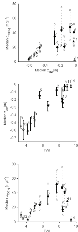
Fig. 6. Links between median groundwater positions z_{GW} , median flow-weighted TOC profile concentrations ( c_{TOC,q} ) and the topographic wetness index (TWI). In the upper plot (a) median flow-weighted c_{TOC,q} values (from 9 sampling occasions in 2008–2009) are plotted against median z_{GW} values. The middle plot compares median z_{GW} values against the TWI whereas the lower plot compares median c_{TOC,q} values against the TWI. Vertical error bars show the 10th and 90th percentile groundwater positions (b) respectively the potential range of flow-weighted TOC concentrations (a,c) assuming average profile concentrations (solid lines) or changing profile concentrations (dotted lines). Circles represent sites located in the till parts and triangles represent sites located in the sedimentary part of the catchment. Organic sites are colored black, mineral sites are white and mineral-organic sites are grey. Site numbers are plotted next to the circles and triangles. Only site numbers are shown and “R” prefixes used in the text (preceding the site digits) were omitted for better readability.
