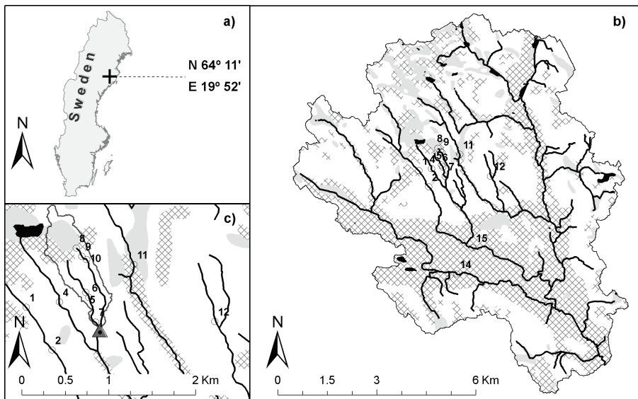
Fig. 1. Locations of the (numbered) riparian monitoring sites (empty white circles) in the Krycklan catchment (outlined by thin black lines in inset b ) and the gauging station (black triangle) at the outlet of Svartberget (outlined by thin black lines in inset c ). Streams and lakes are represented by black areas and thin black lines. Parts of the catchment underlain by till are shown as white areas and others underlain by alluvial sediment deposits are marked by the cross-hatched areas respectively while wetlands are highlighted as grey shaded patches. Wetlands and lakes are highlighted as grey patches. Only site numbers are shown and “R” prefixes used in the text (preceding the site digits) were omitted for better readability.
