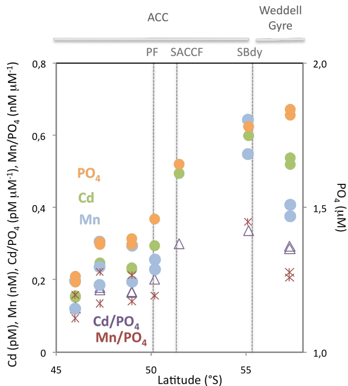
Fig. 6. Variations of Cd, Mn, PO 4 concentrations, and of Cd/PO 4 and Mn/PO 4 ratio as a function of latitude in the surface waters (>60 m) of the Antarctic Circumpolar Current and the northern Weddell Gyre along the Greenwich Meridian.
