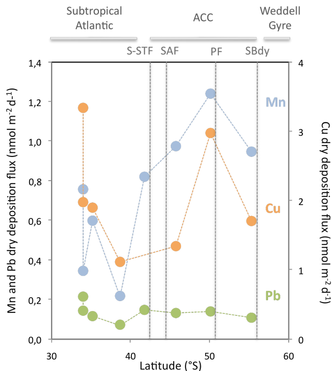
Fig. 4. Dry deposition flux of Mn, Cu and Pb (in \text{nmol m}^{-2} \text{d}^{-1} ) as a function of latitude along the section in the southeastern subtropical Atlantic and the Southern Ocean. An estimated dry deposition velocity of 0.3 \text{ cm s}^{-1} was used to calculate the fluxes. Ag and Cd dry deposition fluxes were extremely low along the section: from <0.06 \text{ nmol m}^{-2} \text{d}^{-1} in the northernmost part of the section to <0.02 \text{ nmol m}^{-2} \text{d}^{-1} in the southern side of the ACC for Ag, and below 0.05 \text{ nmol m}^{-2} \text{d}^{-1} in the northernmost area to <0.01 \text{ nmol m}^{-2} \text{d}^{-1} in the southern side of the ACC for Cd.
