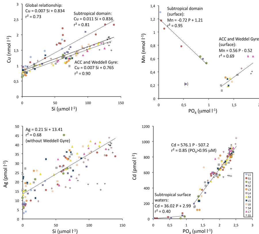
Fig. 5. Relationships among Cu, Ag, Mn and Cd concentrations, and silicic acid (Si)-left panels or phosphate (PO 4 )-right panels concentrations along the section between the southeastern Atlantic and the Southern Ocean.
