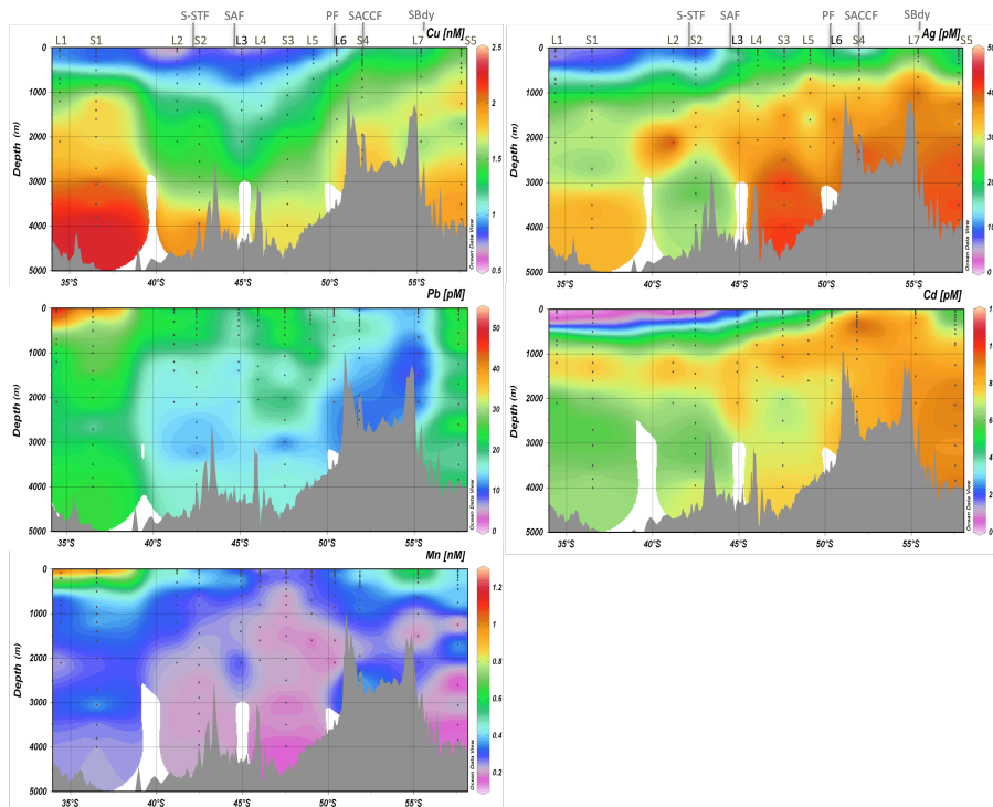
Fig. 3. Contour plots of dissolved copper (Cu), silver (Ag), lead (Pb), cadmium (Cd) and manganese (Mn) along the MD166 BONUS-GoodHope section between the southeastern Atlantic and the Southern Ocean. The positions of L and S stations and the fronts are indicated. The colour mapping extrapolation is based on the sampling resolution along the section of \sim 2600 km that was achieved with 12 stations separated on average by \sim 2.2^\circ latitude, with a total of 160 sampling depths. Figure from ODV (Reiner Schlitzer).
