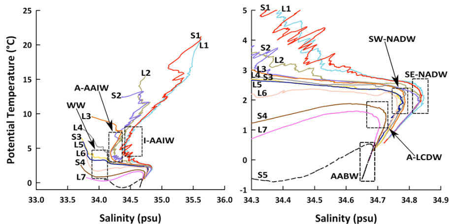
Fig. 2. Diagrams of salinity (psu) versus potential temperature (°C) in the whole water-column (left panel) and in deep waters (right panel) at the stations sampled for trace metals determination (CTD data and validation from Branellec et al., 2010; Kermabon and Arhan, 2008).
