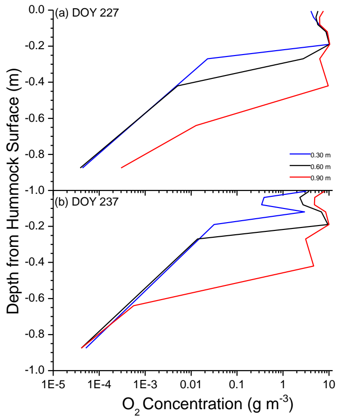
Fig. 11. Vertical profiles of aqueous O_2 concentration ( [O_{2s}] ) modelled below hummocks on DOY 227 and 237 in 2002 by raising or lowering the depth of the external water table from 0.6 m (Fig. 1) to 0.3 m or 0.9 m.
