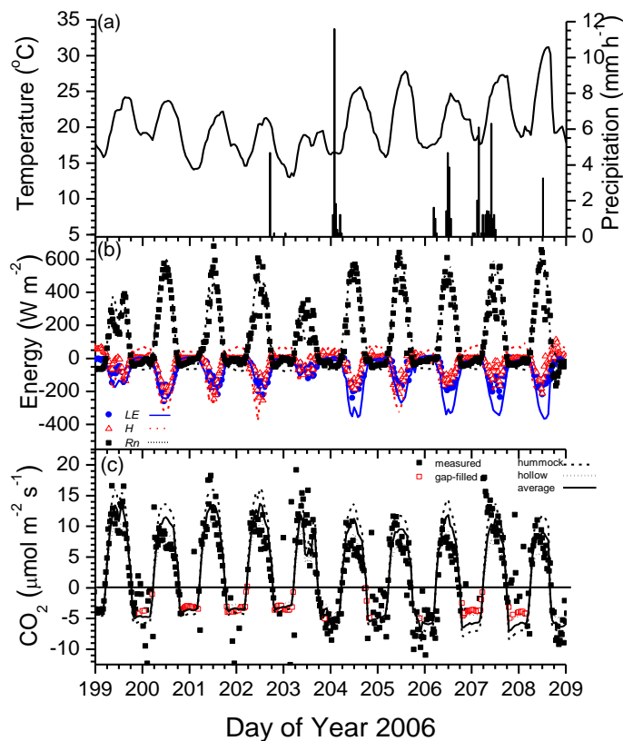
Fig. 7. Air temperature and precipitation, and energy and \text{CO}_2 fluxes measured (symbols) and modelled (lines) before and after precipitation events with a low water table from DOY 200 to 209 in 2006 (0.7 m in Fig. 2). Positive values represent downward fluxes, negative values represent upward fluxes.
