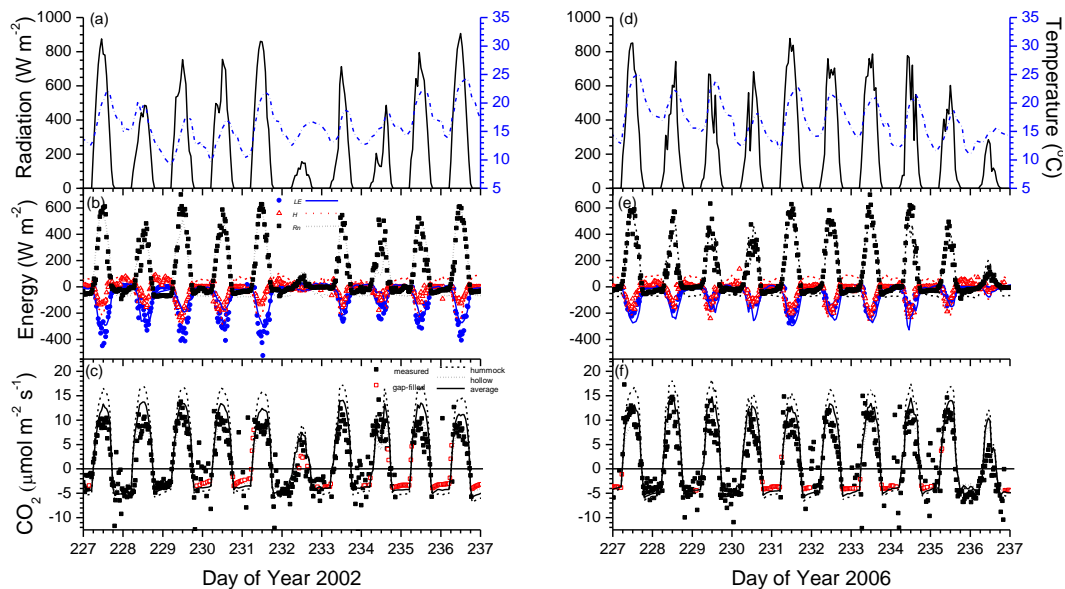
Fig. 4. Radiation and air temperature, energy and \text{CO}_2 fluxes measured (symbols) and modelled (lines) from DOY 228 to 237 with high water table in 2002 (0.2 m in Fig. 2) and low water table in 2006 (0.7 m in Fig. 2). Positive values represent downward fluxes, negative values represent upward fluxes.
