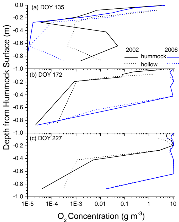
Fig. 8. Vertical profiles of aqueous O_2 concentration ( [O_{2s}] ) modelled below hummocks and hollows on DOY 135, 172 and 227 of 2002 and 2006.
