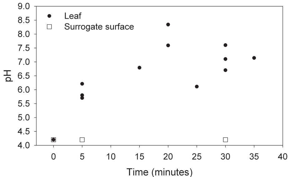
Fig. 8. Time series of pH during controlled leaf droplet experiment. Black dots represent pH of droplets applied to leaves and open squares represent pH of droplets applied to clean Teflon surface. Droplets of pH 4.2 consisting of deionized water and phosphorous acid were applied at t = 0 .
