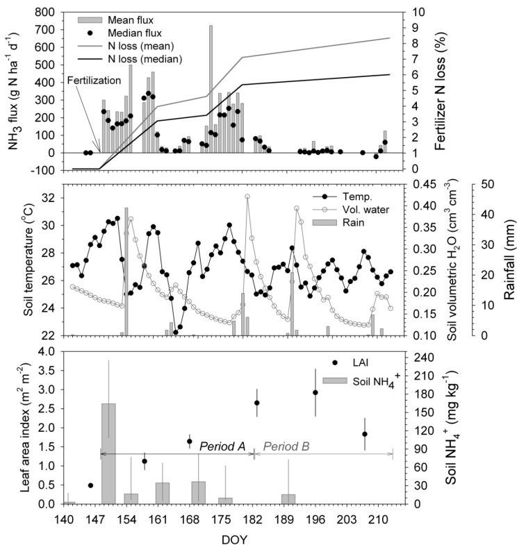
Fig. 4. Daily mean and median \text{NH}_3 fluxes along with equivalent % N loss of applied fertilizer (top graph); daily average soil temperature averaged over 4–8 cm depth, soil volumetric water at 10 cm depth, and rainfall (middle graph); and single-sided leaf area index (LAI) and soil extractable \text{NH}_4^+ concentrations (0–5 cm depth) (bottom graph). Error bars in bottom graph represent \pm 1 standard deviation of the mean. DOY represents the Julian day of the year.
