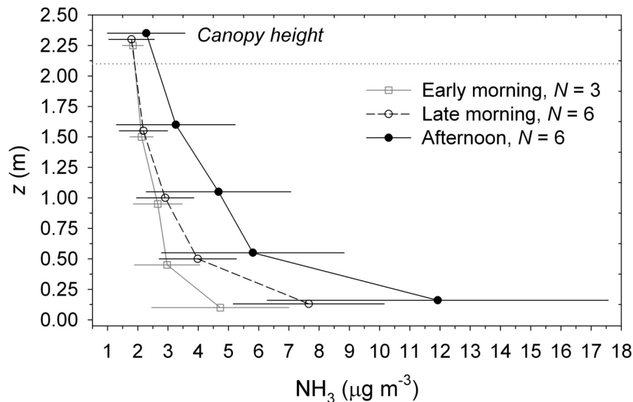
Fig. 9. In-canopy \text{NH}_3 concentration versus measurement height above the ground ( z ). Symbols represent the mean and error bars represent \pm 1 standard deviation of the mean. Lines connecting observations are included only as a visual aid. “Early morning” includes profile measurement periods ending before 09:00, “late morning” includes profile measurement periods ending between 09:00 and 13:00, and “afternoon” includes profile measurement periods ending between 13:00 and 18:00.
