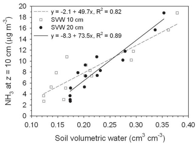
Fig. 10. Time series of soil volumetric water during in-canopy measurement period along with \text{NH}_3 air concentration at z = 10 cm above the soil surface (top graph); correlation between \text{NH}_3 concentration at z = 10 cm and soil volumetric water at 10 and 20 cm depth (bottom graph).
