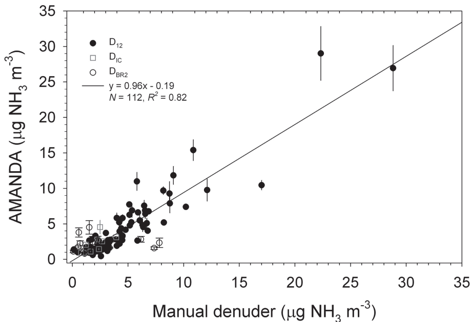
Fig. 3. Comparison of AMANDA \text{NH}_3 concentration measurements to 12-h ( D_{12} ) integrated samples, 2–3 h samples from the in-canopy profile system ( D_{1C} ) and 2 h samples from the second Bowen ratio system ( D_{BR2} ). Concentrations were normalized to a common level using the linearized concentration gradient ( dC/d\ln z ) to account for differences in measurement heights. Error bars represent \pm 1 standard deviation of the mean half-hourly AMANDA measurements.
