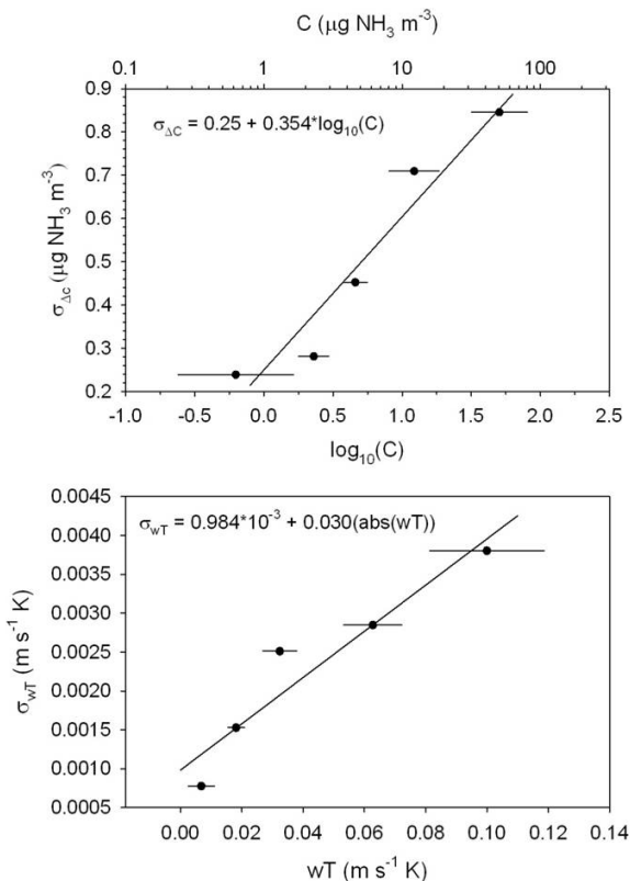
Fig. 1. Summary of relationships used to derive precision estimates of AMANDA NH 3 gradient ( \sigma_{\Delta C} ) and kinematic heat flux ( \sigma_{wT} ) measurements from which the uncertainty of the modified Bowen-ratio NH 3 flux was calculated. In the top graph, upper and lower x axes represent NH 3 air concentration and log-transformed concentration, respectively. In the lower graph, the x-axis represents the kinematic heat flux. Symbols represent bin-wise average values and error bars represent \pm 1 standard deviation of x .
