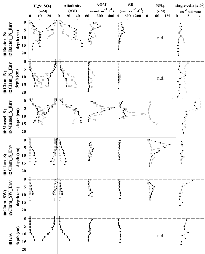
Fig. 3. Geochemical depth profiles of \text{H}_2\text{S} , \text{SO}_4 , AOM, SR, \text{NH}_4 , alkalinity and single cell counts at all investigated sites at REGAB. Closed symbols denote measurements taken within the patches/bacterial mat, and open symbols denote measurements taken at the nearby bare sediments. N.d. = not determined.
