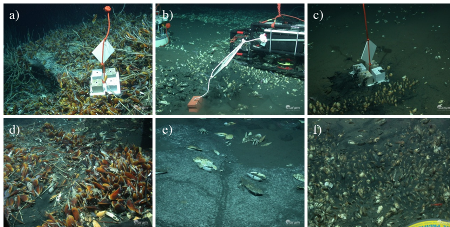
Fig. 2. Typical habitats at the REGAB pockmark: the central area with extensive carbonate crust and outcropping hydrates populated by mussels and tubeworms (a) ; clam patches overlying blackened reduced sediment (b, c, f) ; mussel patch on soft sediment (d) ; white bacterial mat at the REGAB_N (e) ; Benthic chamber incubation is visible in (b) picture.
