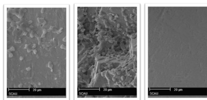
Figure S1 SEM images of the pyrite cube surfaces under different treatments. (a) exposed to Acidithiobacillus ferrooxidans only; (b) exposed to Acidithiobacillus ferrooxidans and 50 µM H 2 O 2 ; and (c) exposed to Acidithiobacillus ferrooxidans and 100 µM H 2 O 2 . Arrows point to the cells attached to the surfaces of pyrite crystals.
