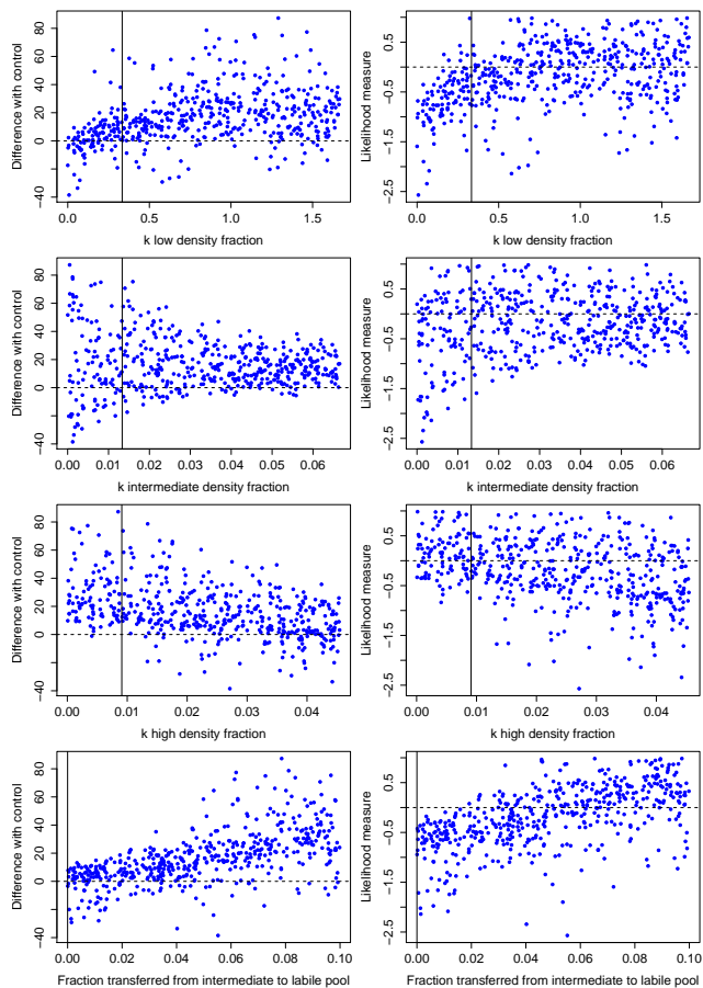
Fig. 2. Dotty plots generated by randomly modifying the values of the decomposition rates and the transfer from the intermediate pool to the labile pool. Additional details are provided in the manuscript.
