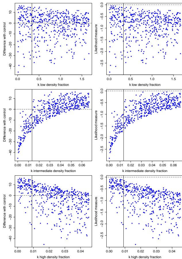
Fig. 1. Dotty plots generated by randomly modifying the values of the decomposition rates of the different fractions by a factor between 0 and 5. Additional details are provided in the manuscript.
