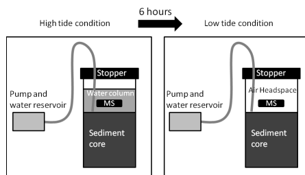
Fig.1 Diagram of the experimental setup, showing the conditions of simulated tides. TA and DIC are sampled from the water column during inundation (high tide) and CO 2 is sampled from the headspace during exposure (low tide). MS refers to a magnetic stirrer bar.
