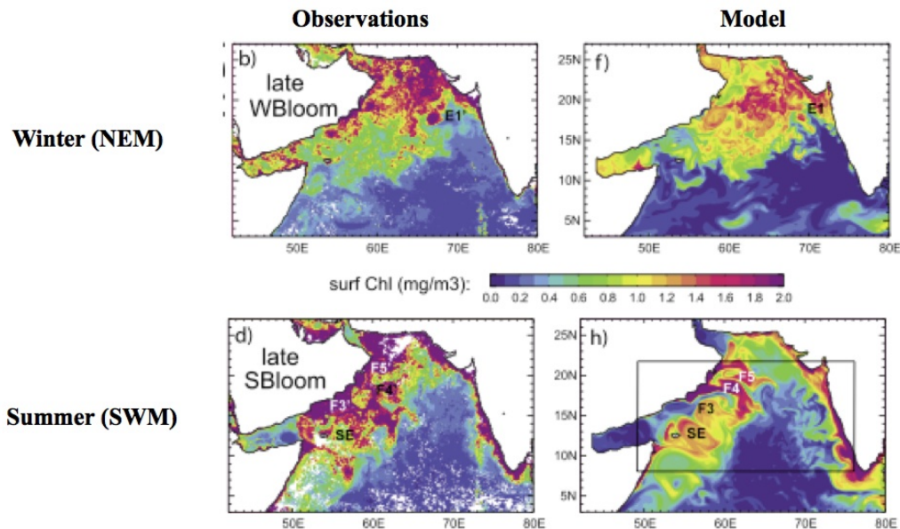
Fig. 3. Snapshots of surface Chl in our model (Resplandy et al., 2011) and satellite observations
