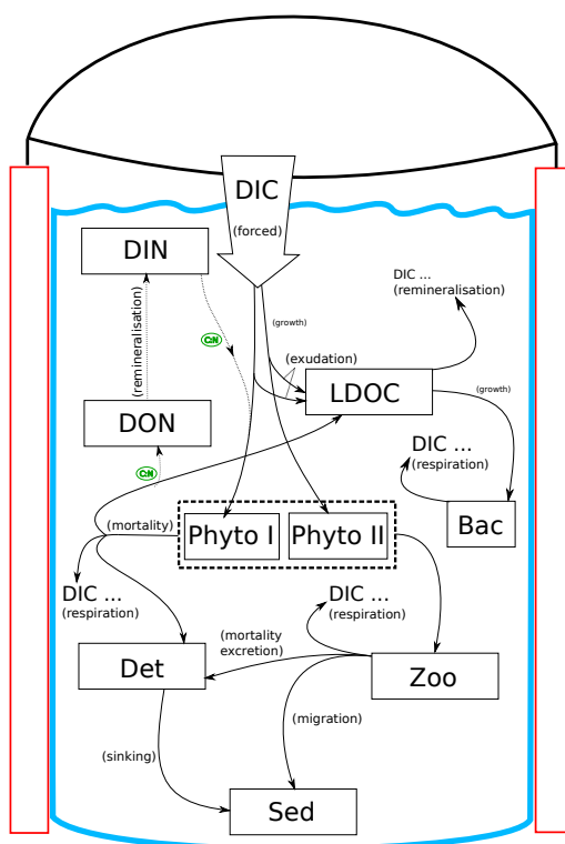
Fig. 1. Conceptual model. Apart from the bacterial (Bac) and zooplankton (Zoo) compartment, all compartments are modeled by two state variables: \text{C}^{13} , and \text{C}^{12} .
