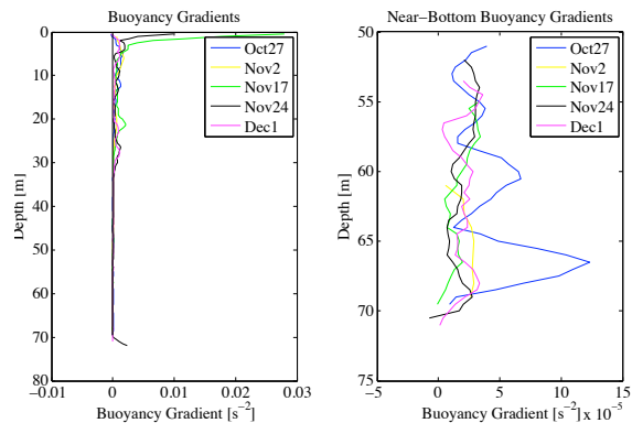
Left: N^2 over the entire basin during the sampling period in 2010. Black line drawn at 0. Right: N^2 over the deep basin during the sampling period.
