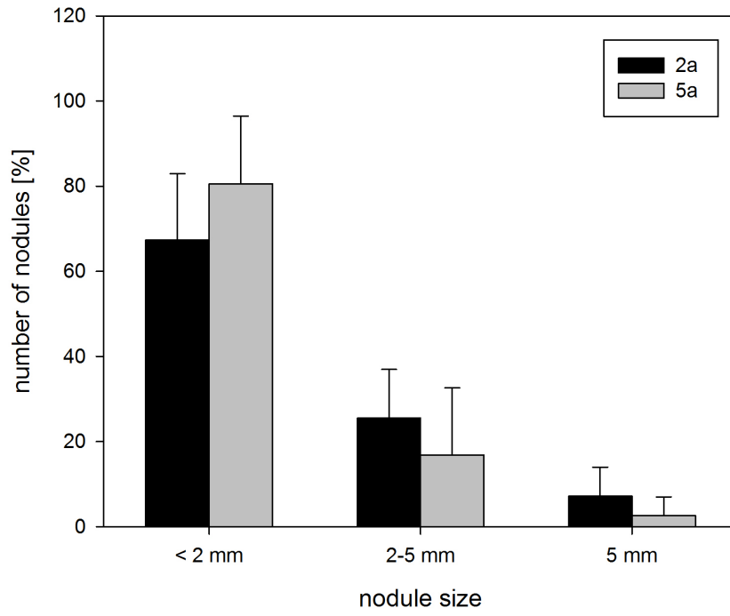
Fig. 2. Distribution of the different nodule size classes, including 9 plants per plot.
