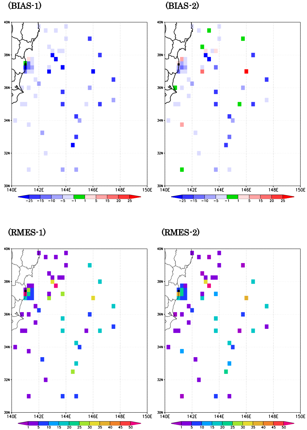
Fig.R1. (new Fig.11) Gridded distributions of mean error (BIAS) and root mean square error (RMSE) between the simulated and observed ^{137}\text{Cs} surface concentration for the period from 21 March to 6 May 2011, normalized by the measurement errors (See Table 1). Grid resolution is 1/4^\circ . The position of FNPP is denoted by a closed square. Left (right) panels denote the JCOPE-T-2-C (JCOPE-T-2-C-E) case.
