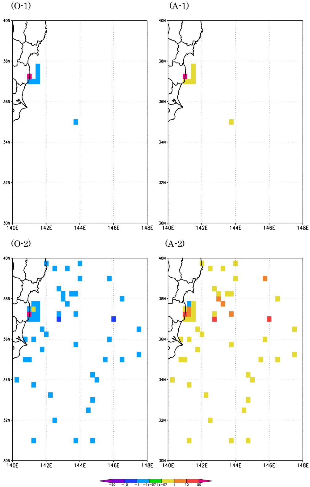
Fig.R3. Contribution rates (in %; Eq. 9) averaged in 1/4^\circ \times 1/4^\circ grids. (O-1) The ocean parameter in the JCOPE-T-2-C case for the period from 21 to 31 March 2011. (A-1) As in (O-1) except for the atmospheric parameter. (O-2) As in (O-1) except for the period from
