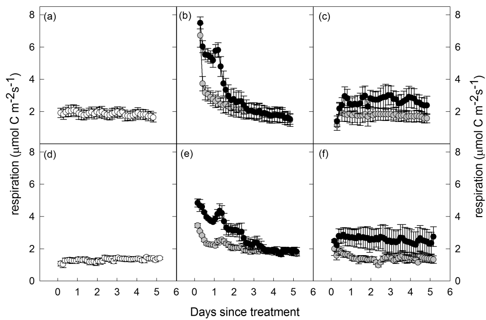
Figure 1: Revised Figure 1. Reference site Experiment 1 (top row) and Experiment 2 (bottom row) respiration in (a,d) control, (b,e) mineral soil, and (c,f) litter surface applications. Light grey symbols indicate water-only and black symbols indicate sucrose+water treatments.
