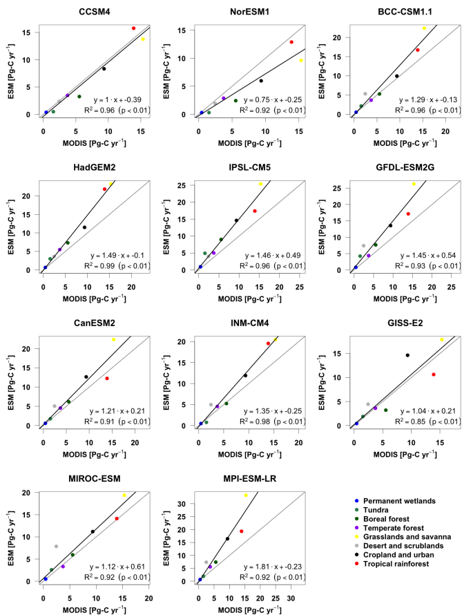
Fig. 3. Biome comparison between Earth system model NPP and MODIS NPP (simulated 1995-2005 mean).
