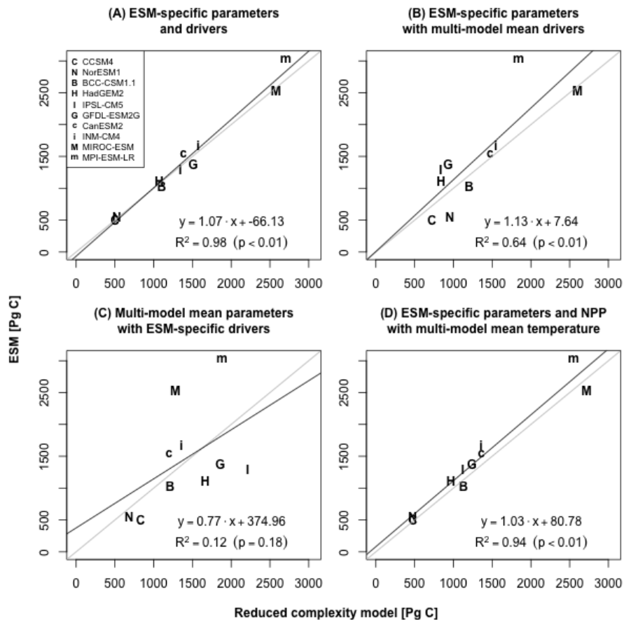
Fig. 1. Explanation of soil carbon stocks across Earth system models (ESMs) by reduced complexity model.
