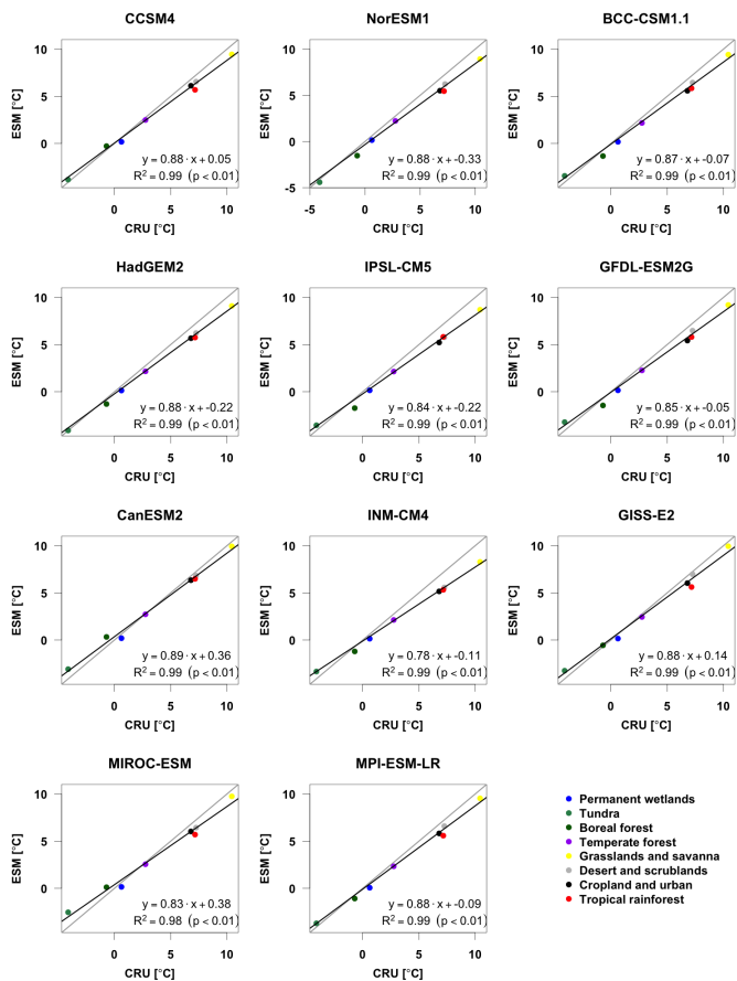
Fig. 2. Mean simulated air temperature (2 m, 1995–2005 mean), versus mean Climate Research Unit (CRU) temperature (2 m, observed 1995–2005) by biome for each Earth system model.
