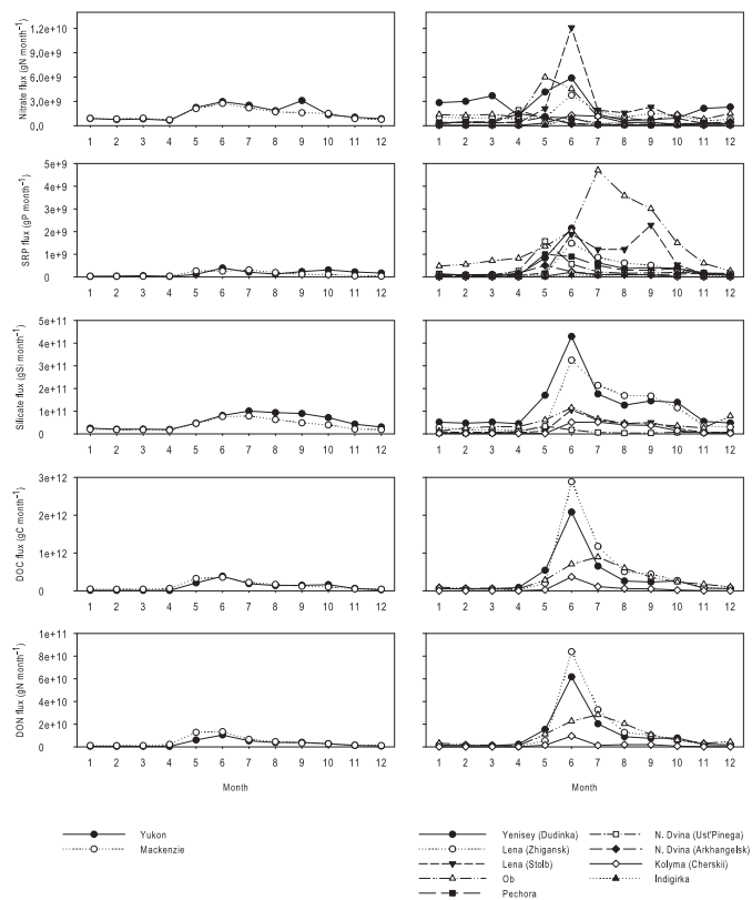
Fig. 3. Monthly flux estimates of riverine nitrate, SRP, silicate, DOC and DON for the North-American and Eurasian rivers.
