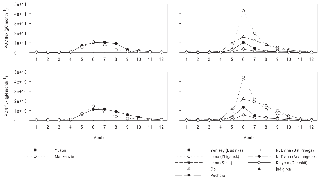
Fig. 4. Monthly flux estimates of riverine POC and PON for the North-American and Eurasian rivers.
