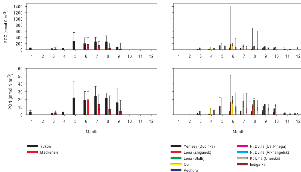
Fig. 2. Monthly-binned concentrations of riverine POC and PON for the North-American and Eurasian rivers. Bars with no standard deviations indicate single values. No filled bars indicate no data available.
