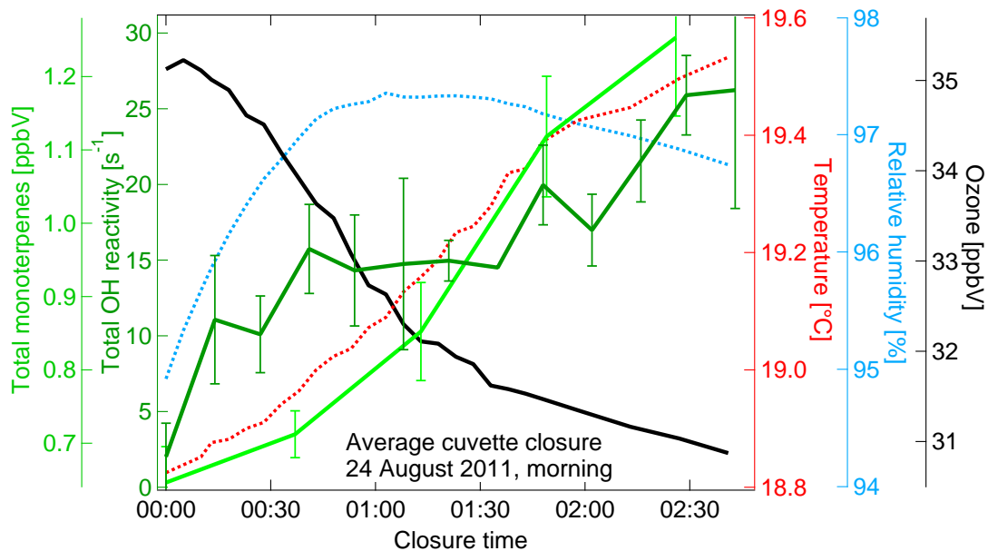
Fig. 1. Example of VOC-PTR-MS (total monoterpenes), CRM (total OH reactivity) and sensor (temperature, relative humidity, ozone) signals inside the cuvette during closures.
