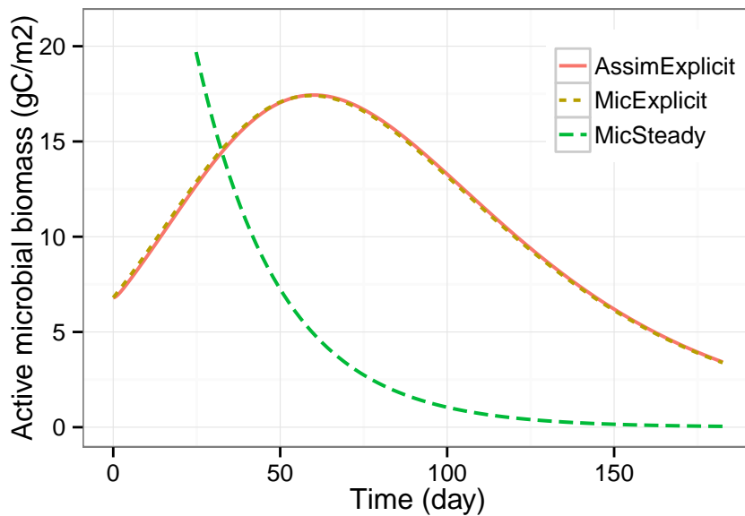
Fig. 1. LabPriming_ActiveMicrobialBiomass
