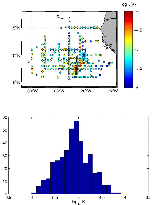
Fig. 2. Upper panel: Map of observed diapycnal diffusivities in the study area. Lower panel: According histogramme of diapycnal diffusivity data
