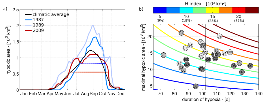
Figure 1: (a) Seasonal dynamics of the hypoxic area for selected years (color plain lines) and climatological average (black plain line). Dotted lines indicate the duration of hypoxia defined by Eq. 2. (b) The H index (colored lines) quantifies the intensity of the seasonal hypoxia event for a given year, and is computed (Eq. 1) as the integral of the hypoxic area over the year, normalized for the average duration of hypoxia (dotted line). The circles locate the hypoxic event diagnosed for each years (1981 -1991 : light gray, 1992-2000 : mid gray and 2001-2009: dark gray) which evidence the variabilities and the lack of relationship between the spatial and temporal extension of hypoxia. H is expressed in units area (if the duration is equal to the average duration, H equates the maximal extension of hypoxia). For inter-site comparability purposes the percentages given below the color bar express H in terms of ratio of the shelf area depicted in Fig. 1.
