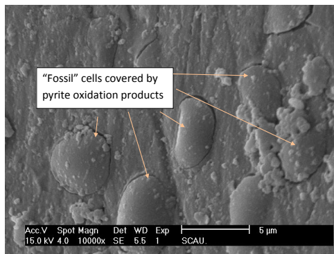
Figure S2 High-resolution SEM image showing the cell-shaped objects observed on the mineral surface in Treatment 1 (T1: \text{H}_2\text{O}_2 at 50 \mu\text{M} ) of Experiment 1. These were the "fossil" cells that were covered by iron oxides/hydroxide/hydroxysulfate formed during attached cell-induced surface corrosion. Note that the size of the cell-shaped object was much greater than the actual size of a cell.
