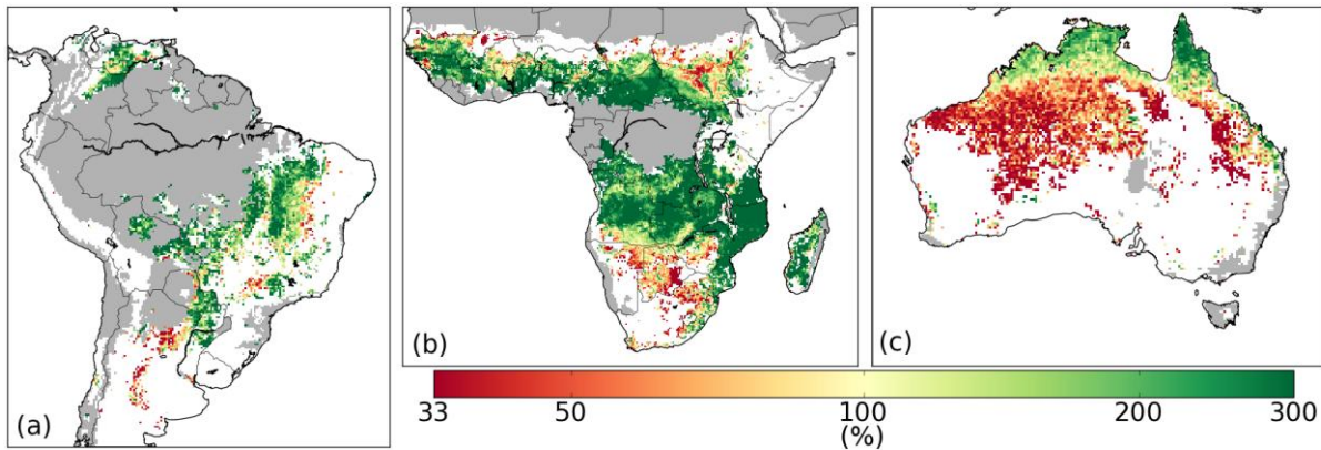
5 Figure 6. Fuel consumption estimated by GFED4s as a percentage of fuel consumption derived here (based on MODIS derived FRE, calibrated against in situ measurements). (a) South America, (b) Sub-Saharan Africa and (c) Australia.
