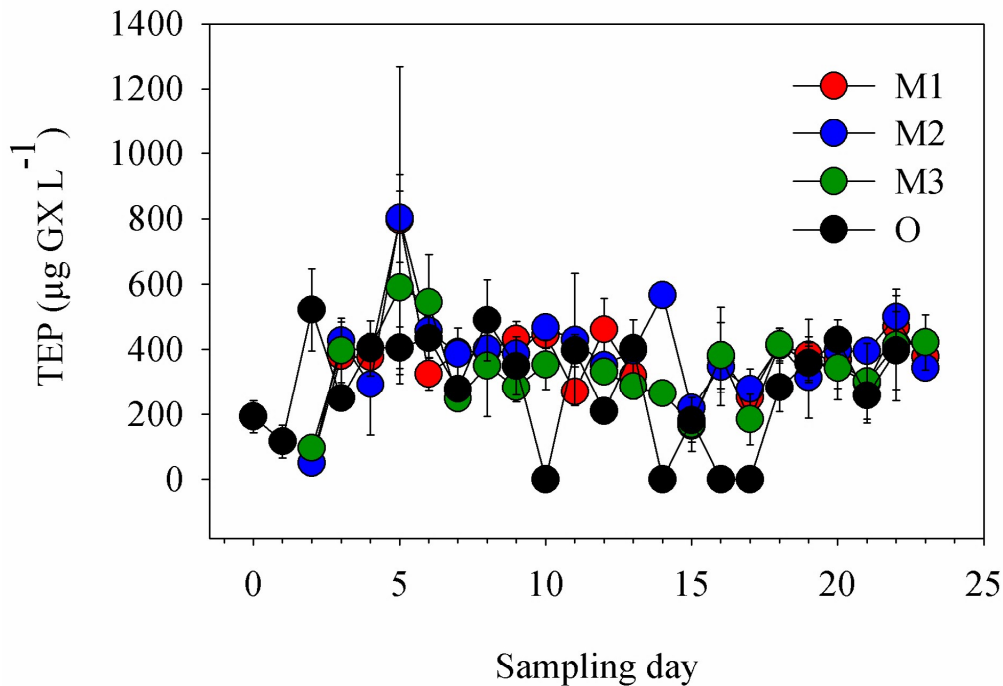
Fig. 1. Temporal dynamics of depth averaged TEP concentrations in all mesocosms (M1, M2, and M3) and lagoon water (O) during the VAHINE experiment
