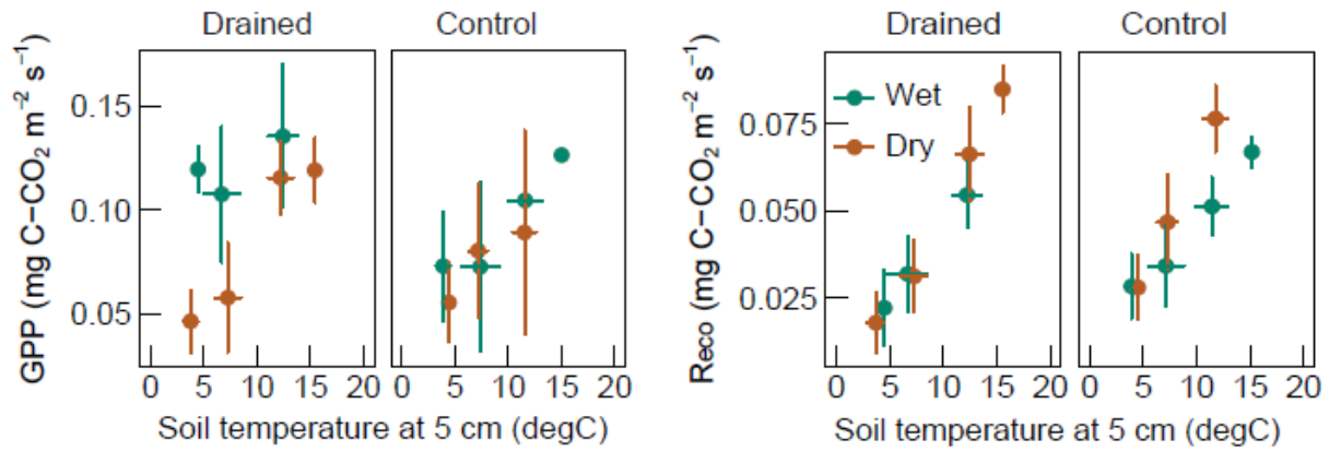
Figure 6 Links between average soil temperatures at 5 cm and gross primary production (GPP) and ecosystem respiration ( R_{\text{eco}} ) rates. Green color indicates wet plots and brown indicates dry plots. Data are from 2013 (20 July–10 August) and sub-season 2014.3 (27 July–20 August); both cover similar phenological periods. Data were grouped into temperature bins of 5 °C.
