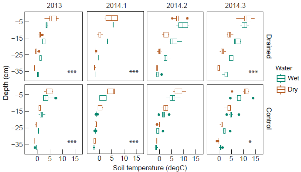
Figure 4 Soil temperature profiles based on observations at 5, 15, 25, and 35 cm depths from even-numbered plots each in the drained (top) and control (bottom) transects. Boxplot contains median, 25 % and 75 % quartiles, and \pm 1.5 interquartile ranges. To minimize the impact of the diurnal temperature cycle on this temporally discontinuous dataset, the time window for averaging was restricted to 1 to 5 pm. Panels from left to right show data from 2013, as well as from three sub-seasons of the growing season of 2014: (2014.1) 15 June–5 July, (2014.2) 6 July–26 July and (2014.3) 27 July–20 August. Green color indicates wet plots and brown indicates dry plots. Data subsets where significant differences in WTD between the wet and the dry plots were detected are marked with asterisks ( P value < 0.001 ***, < 0.01 **, < 0.05 *).
