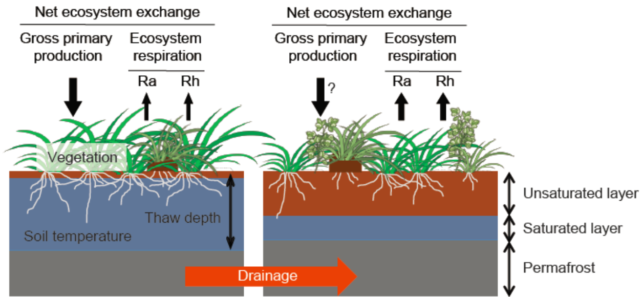
Figure 1 A schematic showing how a decade-long drainage installation affects a floodplain ecosystem and \text{CO}_2 fluxes. Drainage of a floodplain ecosystem alters soil temperatures through changing heat capacity and thermal conductivity, with increased soil temperatures in shallow layers, decreased soil temperatures in deeper layers, and shallower thaw depths; and decreasing the abundance of wetland grasses while increasing the abundance of shrubs. These modifications will subsequently affect \text{CO}_2 fluxes by changing the rates of gross primary production and possibly increasing ecosystem respiration, which consists of autotrophic and heterotrophic respiration ( R_a and R_h ).
