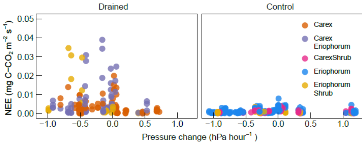
Figure 9 Change in atmospheric pressure and net ecosystem exchange (NEE) from November 2013 by vegetation type (color). Changes in atmospheric pressure refer to changes within 6 hours before individual NEE was measured.
