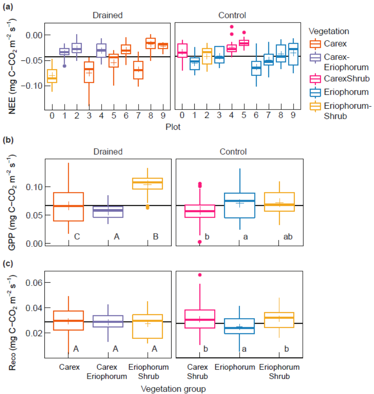
Figure 8 (a) Variability of net ecosystem exchange (NEE) among individual plots during the 2013 growing season. Boxplot contains median, 25 % and 75 % quartiles, \pm 1.5 interquartile ranges, as well as mean values
