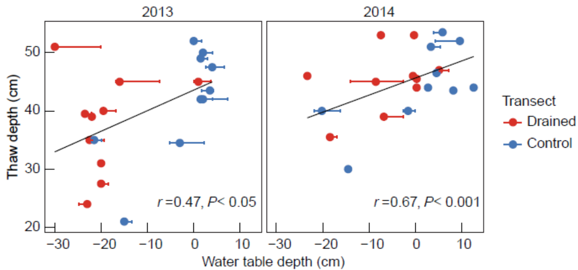
Figure 5 Correlations of thaw depths (TD) and water table depths (WTD) in mid-August 2013 and 2014, where red points indicate plots from the drained transect and, blue points plots from the control transect. Error bars of WTD represent the minimum and the maximum ranges of WTD of the previous 20 days. Results of correlation analysis for each year are presented with black lines.
