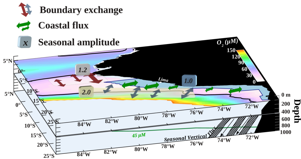
3 Figure 1720. Schematic of the main processes driving the seasonal variability in the SEP OMZ: The 4 oxygen eddy flux through the northern-southern boundaries and the oxygen flux that extends from the 5 coastal boundary into the OMZ. The coastal band limits are defined by the light blue shading adjacent 6 to the coast. A scale of the seasonal amplitude of the eddy driven DO flux at each OMZ boundary is 7 indicated (units in \text{cm s}^{-1} \mu\text{M} ). The position of the 45 \mu\text{M} is also represented (thick black contours). 8 The vertical/offshore oxygen flux induced by the propagation of the annual ETRW across the lower 9 oxycline is represented in the bottom panel. Schematic of the main processes driving the seasonal 10 variability in the SEP OMZ: The DO eddy flux through the northern-southern boundaries and the DO 11 flux that takes place at the coastal boundary of the OMZ. The coastal band limits are defined by the 12 light blue shading adjacent to the coast. A scale of the seasonal amplitude of the eddy driven DO flux at 13 each OMZ boundary is indicated (units in \text{cm s}^{-1} \mu\text{M} ). The mean DO concentration (color shading) and 14 the position of the 45 \mu\text{M} isopleth (thick black contour) at 100 m depth are also represented. The 15 vertical/offshore DO flux induced by the propagation of the annual ETRW across the 45 \mu\text{M} isopleth at 16 25°S is represented in the bottom panel.
