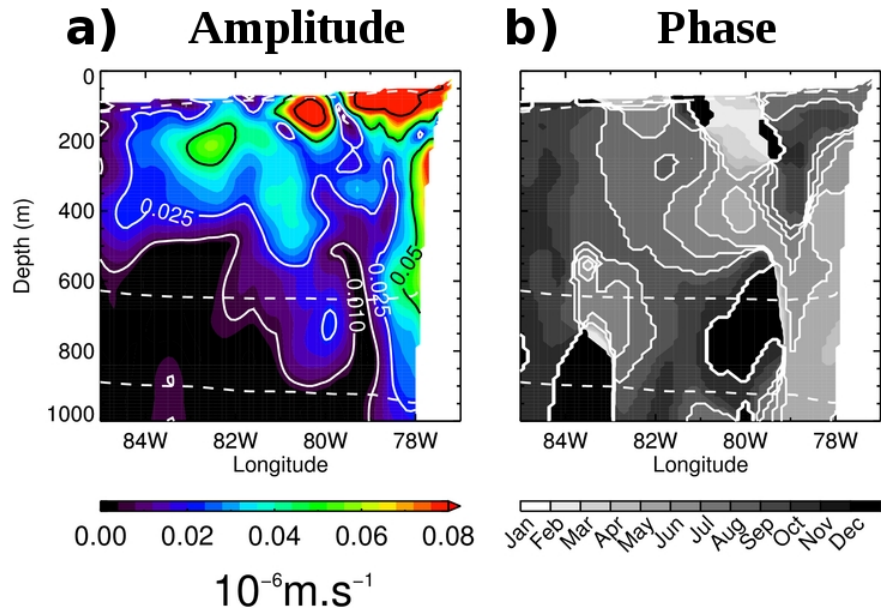
Figure A1. Zonal section of the annual harmonic of the module of the seasonal DO eddy flux vector \langle u' \cdot O_2' \rangle, \langle w' \cdot O_2' \rangle at 12°S. (a) Amplitude of the harmonic and (b) phase of the annual maximum (in months). Dashed white contours indicate the 45 and 20 \mu\text{M} mean DO isopleths. DO was normalized by its RMS prior to carrying out analysis.
