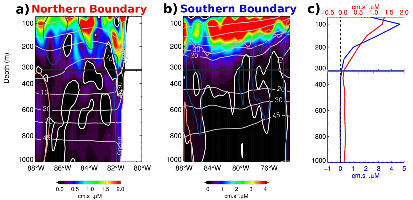
1 Figure 1518. (a) Mean oxygen DO eddy flux normal to the section denoted by the red line in Fig. 2 1417 . (b) Mean oxygen DO eddy flux normal to the section denoted by the blue line in Figure 1417 . (c) 3 Horizontal mean of (a) and (b) (red and blue lines, respectively). Gray contours denote oxygen mean 4 DO concentrations, and light red/blue contours correspond to positive/negative values of mean currents 5 normal to the section ( 1.0/-1.0 \text{ cm s}^{-1} in (a) and 0.4/-0.2 \text{ cm s}^{-1} in (b)). White contour denotes the 0 6 value. The sign convention was chosen so that a positive horizontal flux indicates transport towards the 7 interior of the OMZ.
