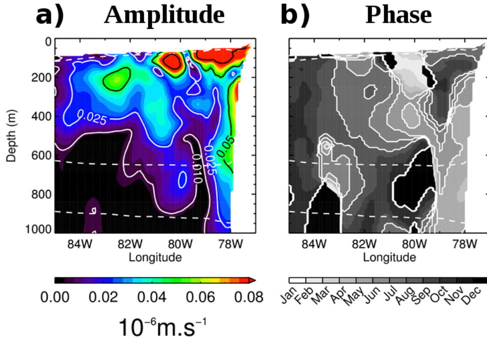
Figure 15. Zonal section of the annual harmonic of the module of the seasonal DO eddy flux vector \left( \overline{\langle u' \cdot O_2' \rangle}, \overline{\langle w' \cdot O_2' \rangle} \right) at 12^\circ\text{S} . (a) Amplitude of the harmonic and (b) phase of the annual maximum (in months). Dashed white contours indicate the 45 and 20 \mu\text{M} mean DO isopleths. DO was normalized by its RMS prior to carrying out analysis. Land and the region outside the 45 \mu\text{M} mean DO isopleth are masked in white.
