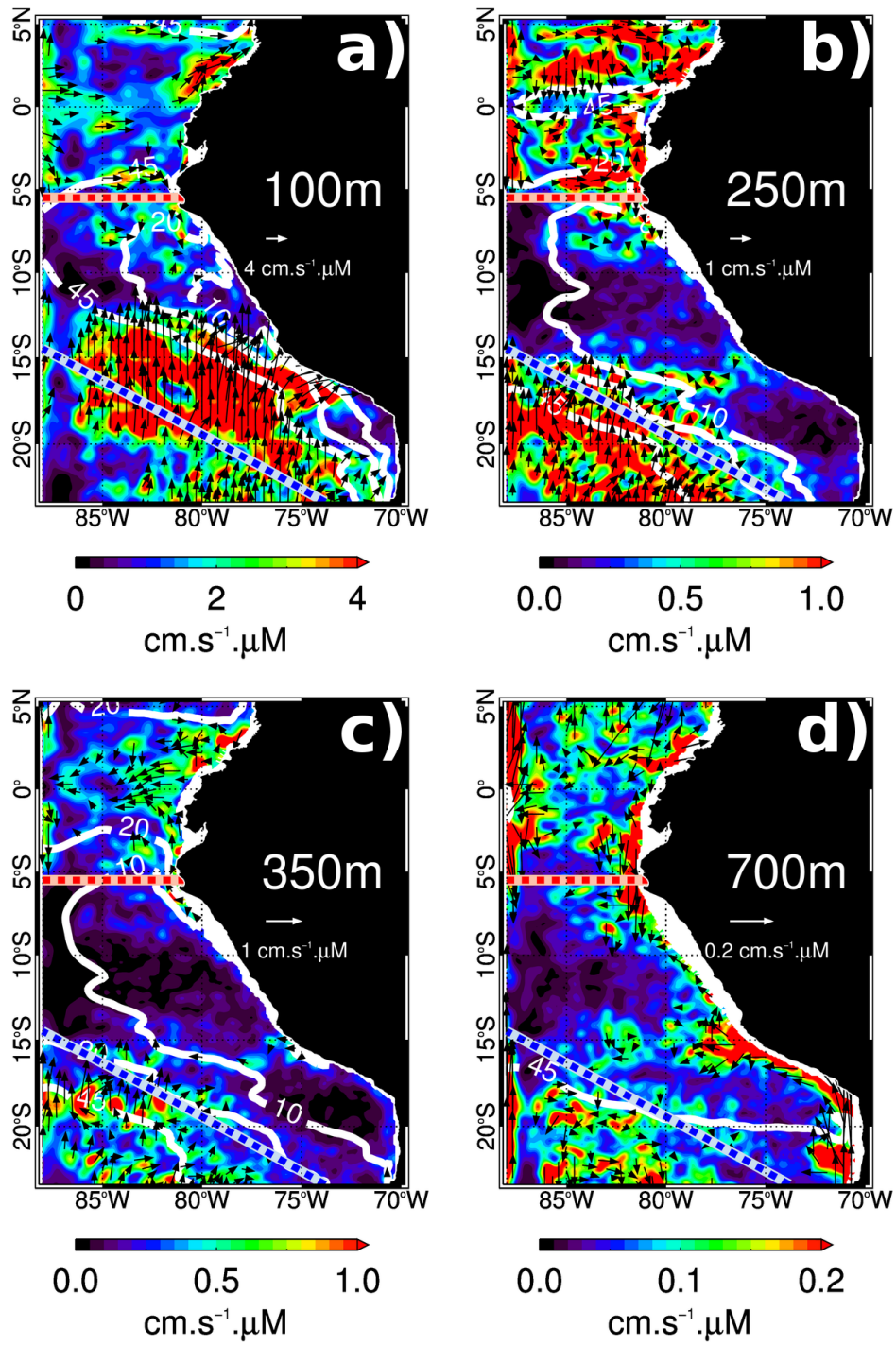
3 Figure 17. Module of the mean DO eddy flux vector \left(\langle u' \cdot O_2' \rangle, \langle v' \cdot O_2' \rangle\right) at (a) 100 m, (b) 250 m, (c) 4 350 m and (d) 700 m depth. Arrows -displayed only for values above the central value in each colorbar- 5 denote the vector direction and strength. White contours correspond to the 45, 20 and 10 \mu\text{M} mean DO 6 values. Red and blue lines denote the position of vertical sections.
