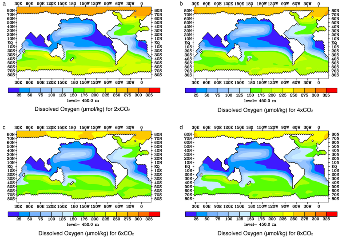
Figure 6. The horizontal expansion of OMZs at 450 meters depth for the Pacific, Atlantic and Indian Oceans in the (a) 2 X \text{CO}_2 simulation, (b) 4 X \text{CO}_2 simulation, (c) 6 X \text{CO}_2 simulation and 8 X \text{CO}_2 simulation.
