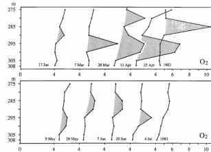
Figure 7. Evolution of dissolved oxygen ( \text{mg}\cdot\text{l}^{-1} ) at SHL 2 on 10 consecutive profiles from January to July 1983, showing persistence of low anomalies during a partial overturn
