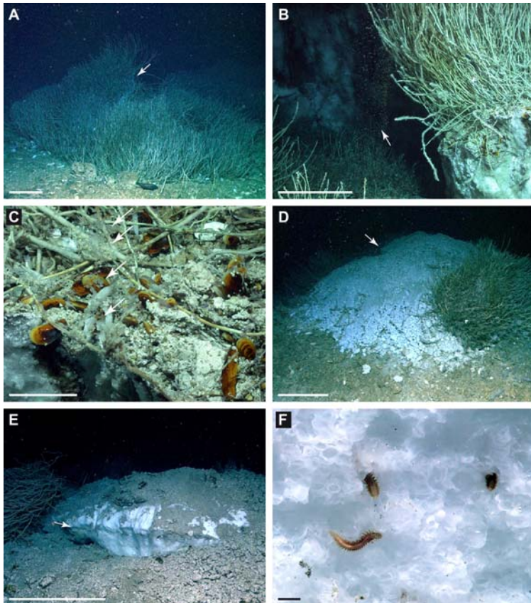
Figure 54. Seafloor images taken at Tsanyao Yang Knoll during ROV QUEST Dive 361. (A) Vestimentiferan tubeworm bushes on a dissected-fractured mound (arrow). Scale bar 50 cm in foreground . (B) Gas bubble plume (arrow) rose through the gap of a dissected-fractured mound. Hydrates formed at the hanging walls. Scale bar 50 cm. (C) Close-up of the mound surface percolated with bubbles emitted into the water column by bubbles (arrows) from the same spot . Gas hydrate occurred below a layer of authigenic carbonates with mytilids, vestimentifera, gastropods, and shrimps on top. Scale bar 10 cm. (D) Mound with outcropping-exposed gas hydrate (arrow) detailed in (E, F). Scale bar 50 cm. (E) Lens-shaped, outcropping exposed gas hydrate composed of bubble-fabric hydrate below and dense hydrate above the arrow. Scale bar 50 cm. (F) Bubble-fabric hydrate inhabited by ice worms (cf. Hesiocaeca methanicola ). Scale bar 1 cm. All images courtesy of MARUM.
