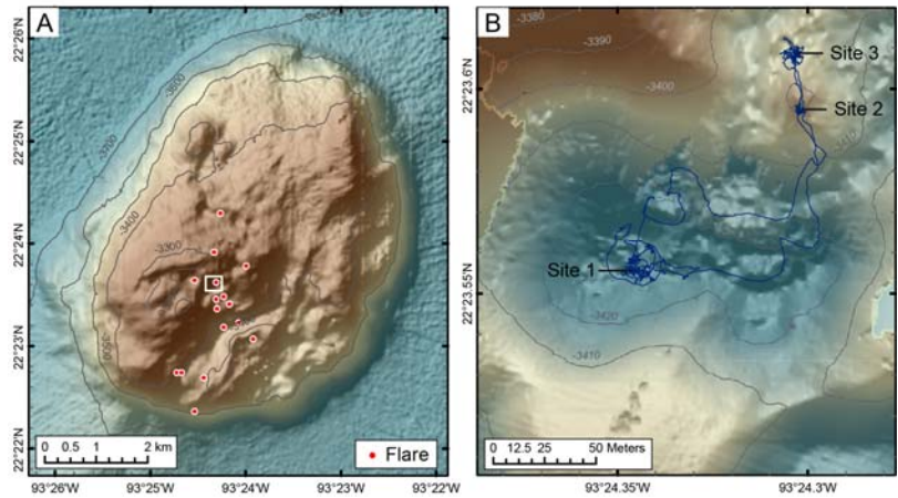
Figure 4. (A) Ship-based swath bathymetry of Tsanyao Yang Knoll (see Fig. 2 for location), flare locations (red dots), and the area shown in (B) (box). (B) ROV QUEST Dive 361 track and the main study sites plotted on AUV swath bathymetry.
