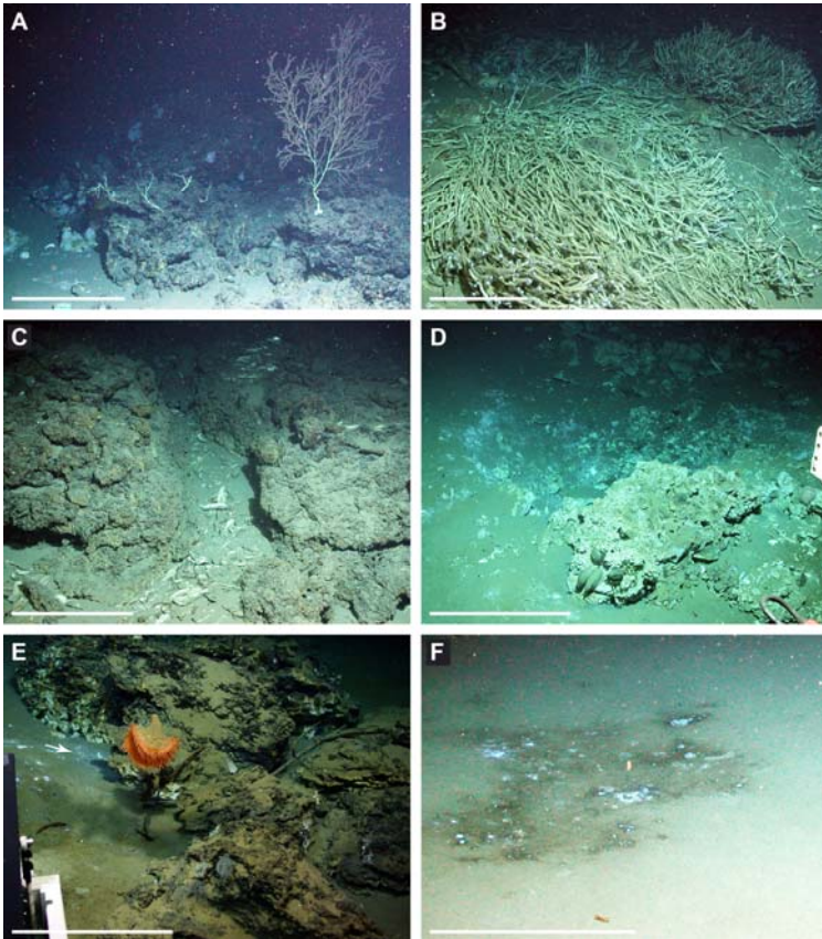
Figure 12.11. Seafloor images taken at UNAM Ridge (A-D) and Knoll 2000 (E-F) during ROV QUEST dives 352 and 353, respectively. (A) Soft coral and other suspension feeders on iron/manganese-stained authigenic carbonates. (B) Recumbent vestimentifera. (C) Authigenic carbonates and mytilid shells. (D) A few living mytilids attached to carbonates (foreground) and a 1 m wide circular depression. (E) Pogonophoran-Frenulate tubeworms were recovered from samples of whitish-stained sediments (arrow) next to carbonates inhabited by suspension feeders ( Actinoscyphia sp., anemones, sponges). (F) Probably whitish patches at seafloor interpreted to be bacterial mats on dark-stained sediments. Scale bar all images 50 cm. All images courtesy of MARUM.
