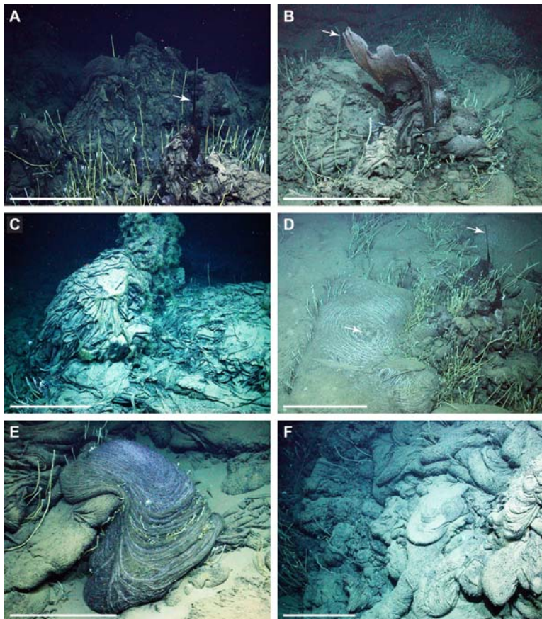
Figure 87. Seafloor images taken at Mictlan Knoll during ROV QUEST Dives 357 (B, C), 363 (A, E), and 364 (D-F). (A-C) Oil whips and sheets (arrows) floating in the water. Old whips and sheets apparently lost buoyancy and pile-up at the seafloor. (D-F) Flow structures of heavy oil. Scale bar all images 50 cm. All images courtesy of MARUM.
