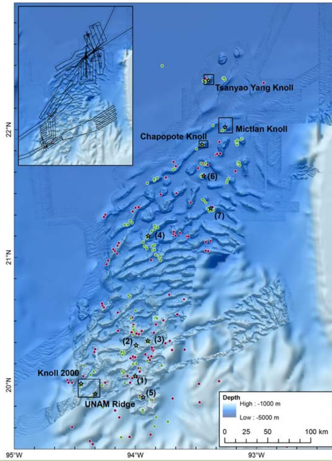
Figure 2. Swath bathymetry draped over GEBCO bathymetry of the Campeche Knolls and cruise track of M 114 (inset). Indicated are oil slick origins as inferred from oil slicks at the sea surface according to Williams et al. (2006) classified as definite (green dots) and probable (grey-purple dots). Seafloor locations of hydrocarbon seepage sites investigated in this study are also shown (open stars, number in brackets). Specifics of those sites are given in Table 1.
