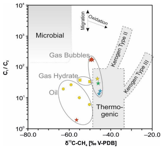
Figure 13.12. Molecular ( C_1/C_2 ) vs. stable C isotopic composition of methane ( \delta^{13}C-CH_4 ) sampled by Gas Bubble Sampler at Tsanyao Yang Knoll (blue), Mictlan Knoll (red), Chapopote Knoll (yellow), and UNAM Ridge (green) and a single oil-associated gas sample (Mictlan Knoll) collected during this study with the GBS. Stars indicate samples analyzed in this study, dots and squares are values according to results for methane in hydrates and oil collected during previous campaigns (MacDonald et al., 2004; Schubotz et al., 2011b). Classification according to the “Bernard diagram” modified after Whiticar (1990). Gas samples studied herein are plotted close to the empirical field of thermogenic methane.
