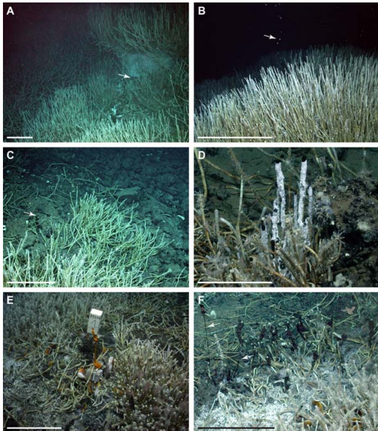
Figure 7.6. Seafloor images taken at Mictlan Knoll during ROV QUEST Dives 357 (A-D) and 360 (E-F). (A) Hydrate below overhanging vestimentiferan tubeworms (arrow). Scale bar 50 cm. (B) Gas bubble stream (arrow) rose through the hydrates and vestimentifera shown in (A). Scale bar 50 cm. (C) Fragmented asphalt, authigenic carbonates (arrow), and vestimentifera. Scale bar 50 cm. (D) Oil drops released through white-coated chimneys. Scale bar 20 cm. (E) Flourishing ecosystem (mytilids, vestimentifera with epizoic suspension feeders, bacterial mats) next to oil-soaked sediments shown in (F). (F) Viscous oil drops emanated from the sediments leaving strands behind (arrow). Scale bar 20 cm. All images courtesy of MARUM.
