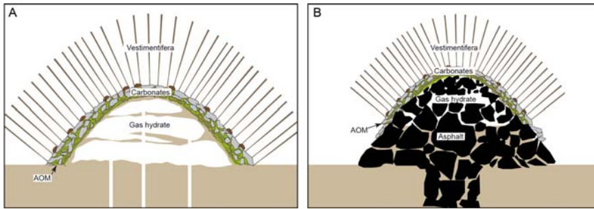
Figure 14.13. Sketch depicting the interpreted vestimentifera-gas/hydrate habitat encountered at (A) Tsanyao Yang Knoll and (B) Mictlan Knoll. Drawing not to scale. The mounds at Tsanyao Yang Knoll were a few meters wide while-whereas Hydrate Hill at Mictlan Knoll was about 30 m in diameter. AOM = anaerobic oxidation of methane (green).
