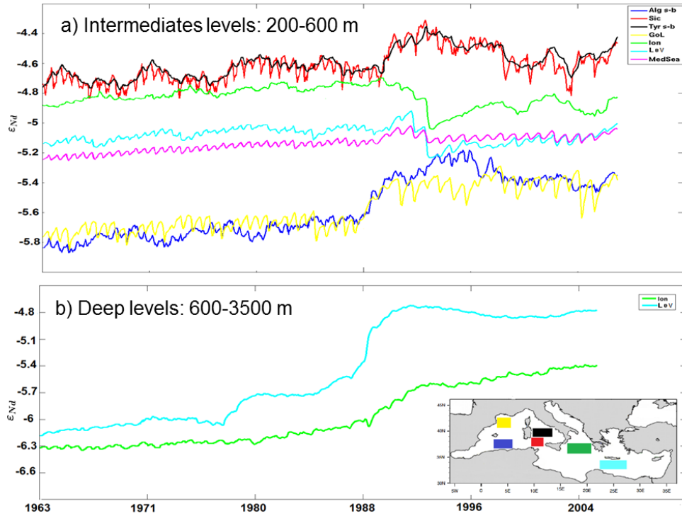
Figure 7. The \varepsilon Nd evolution from EXP2 ( \tau = 3 months) at the intermediate level in (a) (average depth between 200 and 600 m), and for the deep levels in (b) (average depth between 600 and 3500 m). In the Gulf of Lions (yellow), Algerian sub-basin (blue), Levantine s-b (cyan), Ionian s-b (green), Sicily channel (red), Tyrrhenian s-b (black).
