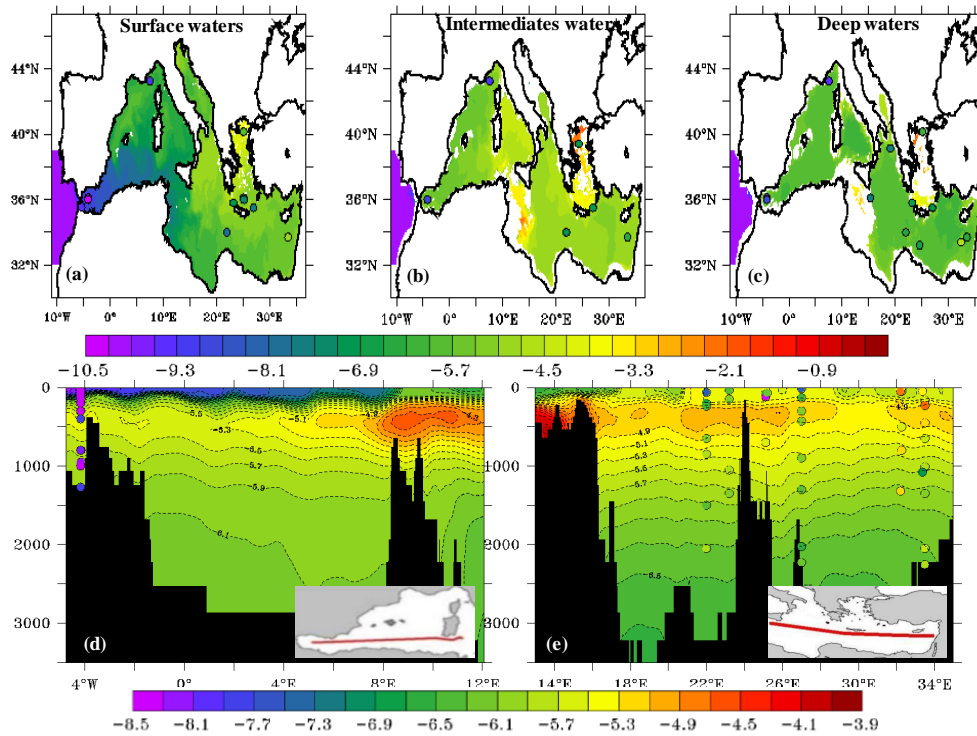
Figure 5. Output of model from EXP2 ( t=3 months) at the steady state. Upper panel: horizontal maps for surface waters (a), intermediate waters (b), and deep waters (c). Lower panel E-W section in WMed (d), and EMed (e), whereas colour-filled dots represent in situ observations from Tachikawa et al. (2004), Vance et al. (2004) and Henry et al. (1994). Both use the same colour scale.
