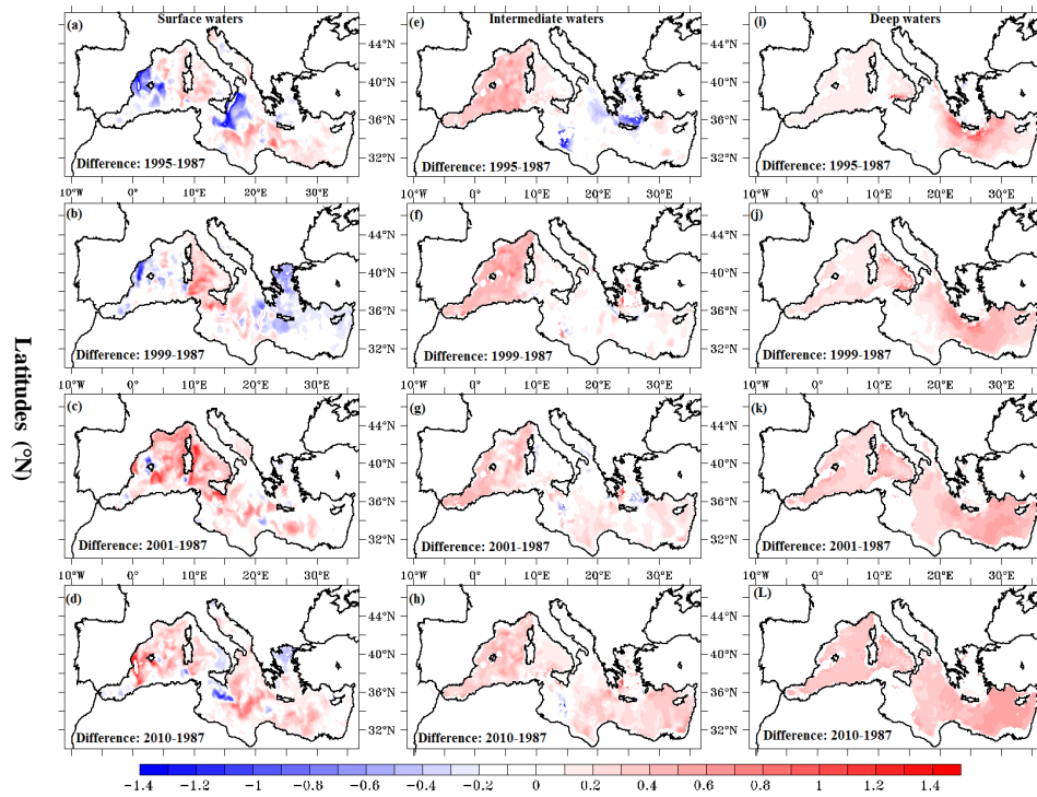
Figure 8. Horizontal maps showing the difference relative to 1987 from EXP2 ( \tau = 3 month), in the left column for the surface level (0 - 200 m), in the middle column for the intermediate layer (between 250 - 600 m), and for the deep layer in the right column (600 - 3500 m).
