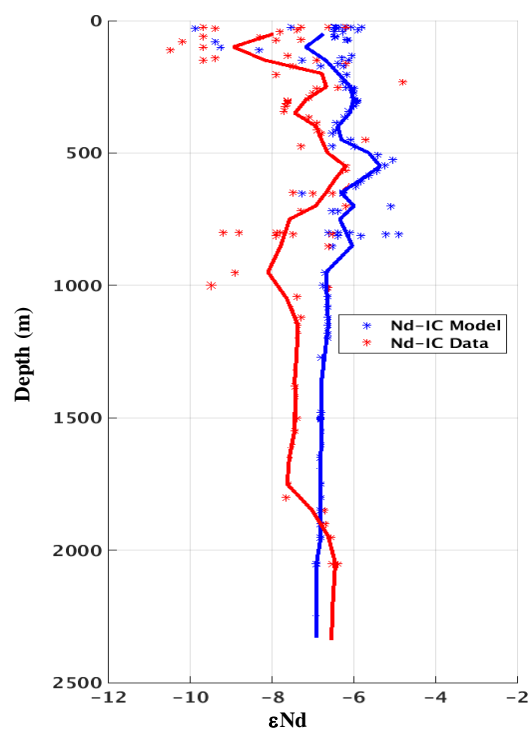
Figure 6. Comparison of average vertical profiles of Nd isotopic signature (Nd-IC) from EXP3 ( t = 3 months) in the whole Mediterranean Sea. Model results are in blue, while red indicates the in situ data.
