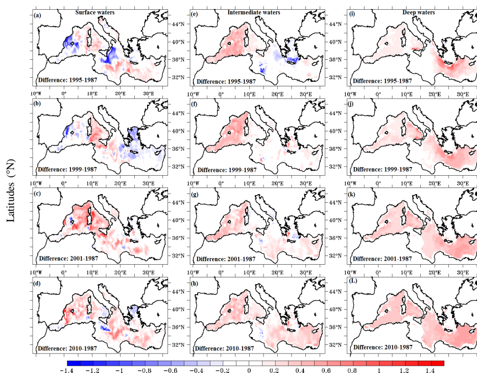
Figure 8. Horizontal maps showing the model output from EXP3 ( \tau = 3 month), in the left column for the surface level (0 - 200 m), in the middle column for the intermediate layer (between 250 - 600 m, and for the deep layer in the right column (600 - 3500 m).
