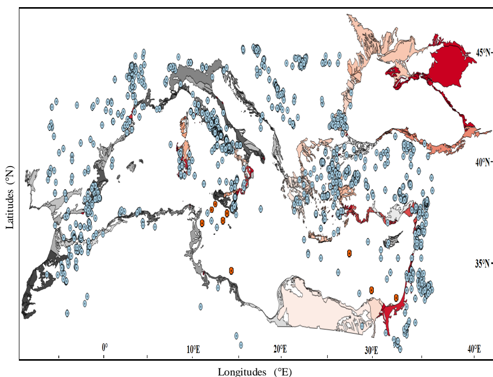
Figure 1. The filled contours indicate the geological province limit from a high resolution digital geological map ( http://www.geologie.ens.fr/spiplabocnrs/spip.php?rubrique67 ) while the circles filled in blue represent the location of the discrete data compiled from EarthChem database (see Appendix 1), and in red the location of the stations corresponding to the sediments analysed as part of the present work.
