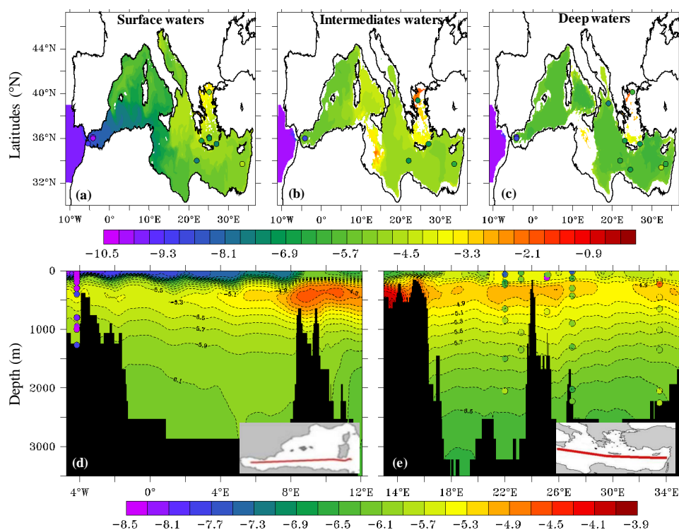
Figure 5. Output of model from EXP3 ( t=3 months) at the steady state. Upper panel: horizontal maps for surface waters (a), intermediate waters (b), and deep waters (c). Lower panel E-W section in WMed (d), and EMed (e), whereas colour-filled dots represent in situ observations (Tachikawa et al., 2004). Both use the same colour scale.
