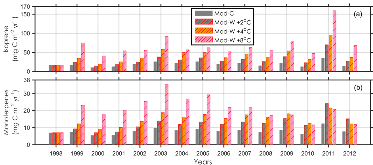
Figure 6 Modelled annual isoprene and monoterpene emissions for the period 1998-2012 at the Abisko heath tundra. The warming (W) treatment started in 1999 and three levels of warming (+2 °C, +4 °C and +8 °C) were applied during summertime. The modelled annual emissions in the control (C) plots are also presented.
