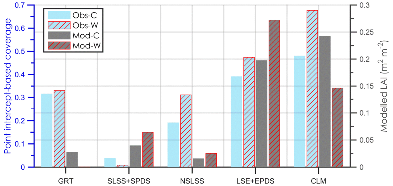
5 Figure 3 Point-intercept based vegetation coverage and modelled leaf area index (LAI, \text{m}^2 \text{m}^{-2} ) averaged for the growing season 2010 and 2012 for the control (C) and warming (W) treatments in the Abisko tundra heath. Different y axes are used for the observed (Obs) and the modelled (Mod) coverage to allow comparison of warming effects. GRT: Graminoid tundra; SLSS: Salix , low shrubs summergreen; SPDS: Summergreen prostrate dwarf shrubs; NSLSS: Non- Salix , low shrubs summergreen; LSE: Low shrubs evergreen; EPDS: Evergreen prostrate dwarf shrubs; CLM: Cushion forbs, lichens and moss tundra.
