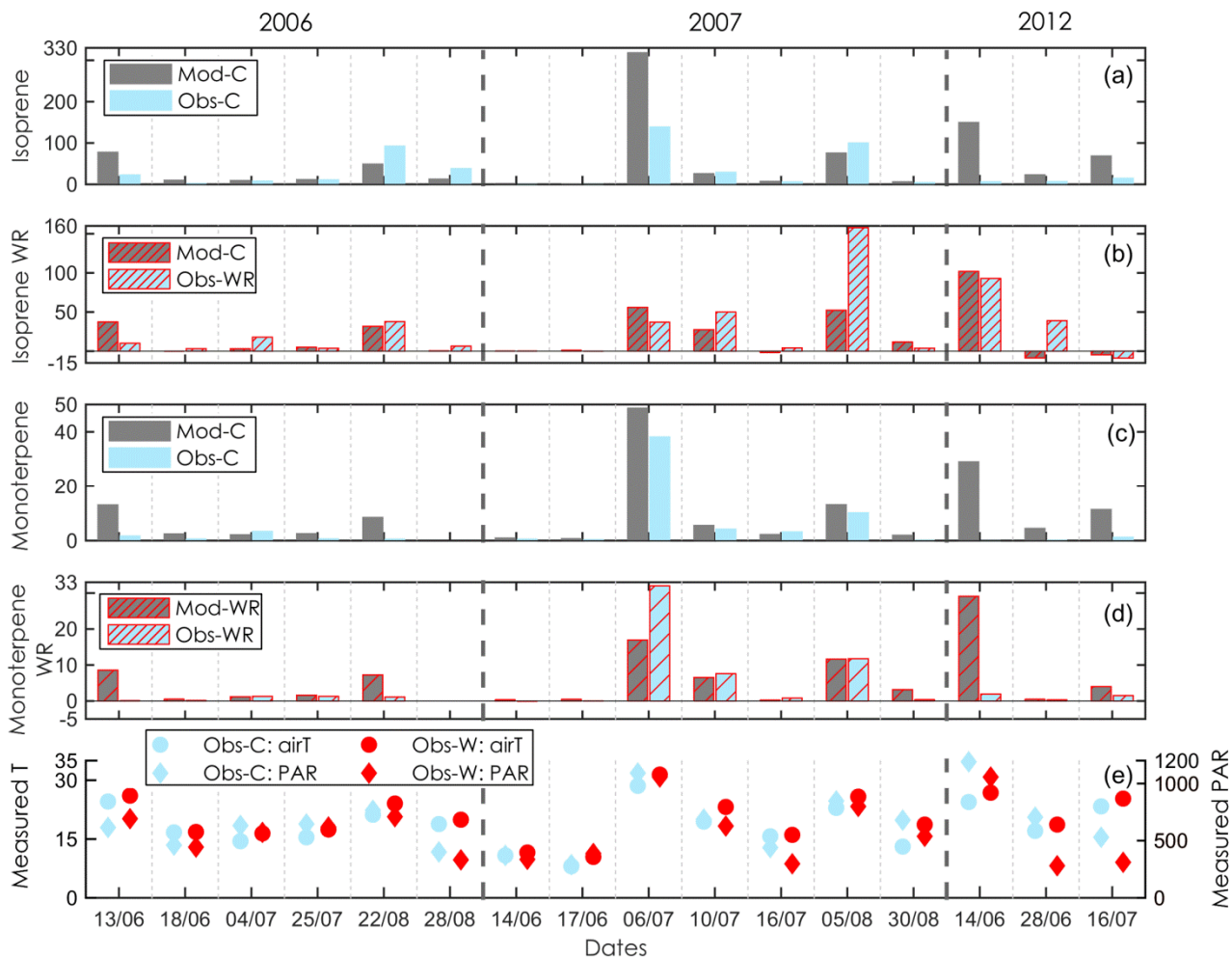
Figure 4 Comparison of the modelled (a) isoprene and (c) monoterpene emission rates with the observations in the control (C) plots and evaluation of modelled warming responses (WR) with the observed WR (b and d) at the Abisko tundra heath. The observed enclosure air temperature (airT) and PAR outside the enclosure are displayed in (e). Mod: Modelled; Obs: Observed.
