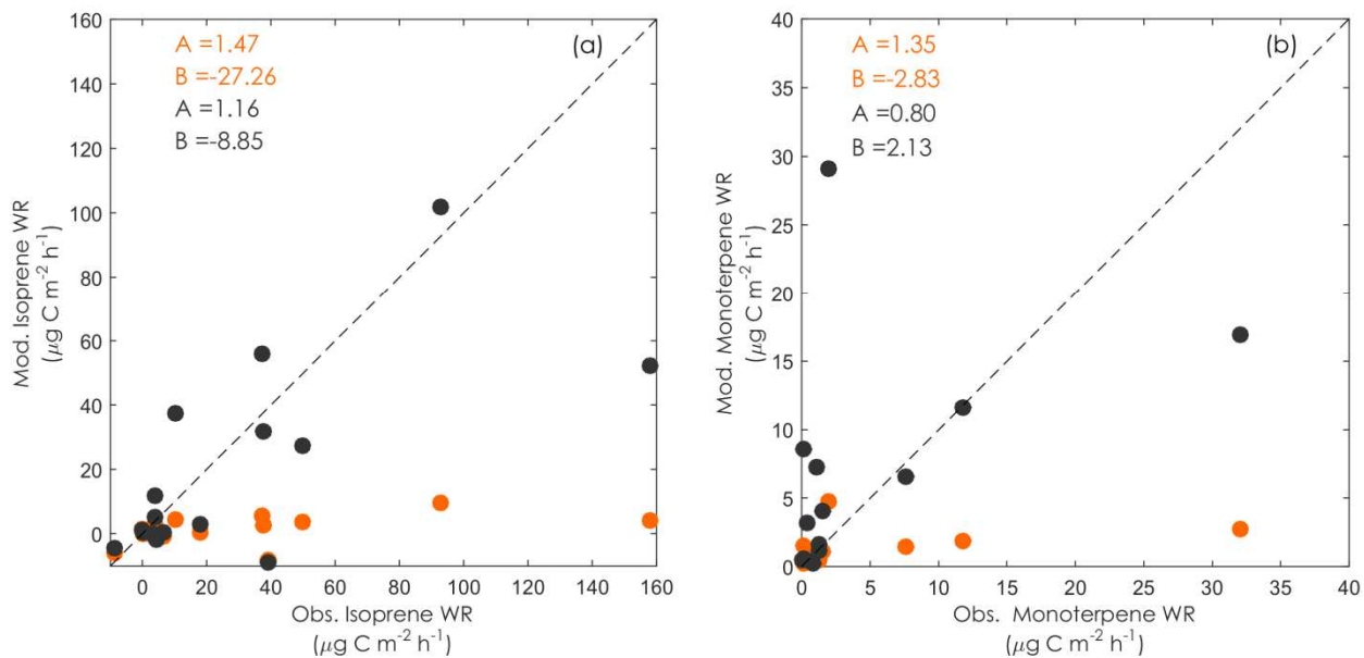
Figure 5 Scatter plot of the modelled (Mod.) and the observed (Obs.) warming response (WR) for both isoprene (a) and monoterpene (b), using the adjusted and the original T response.
