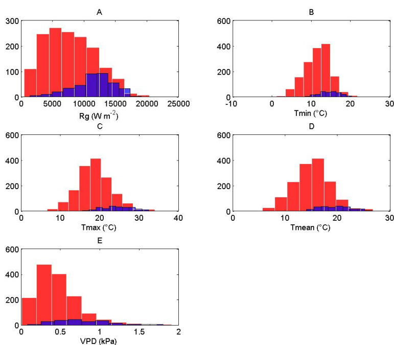
Fig. 1. Histograms of meteorological variables for the trainingsdataset (red) and the high O 3 uptake dataset (blue).
