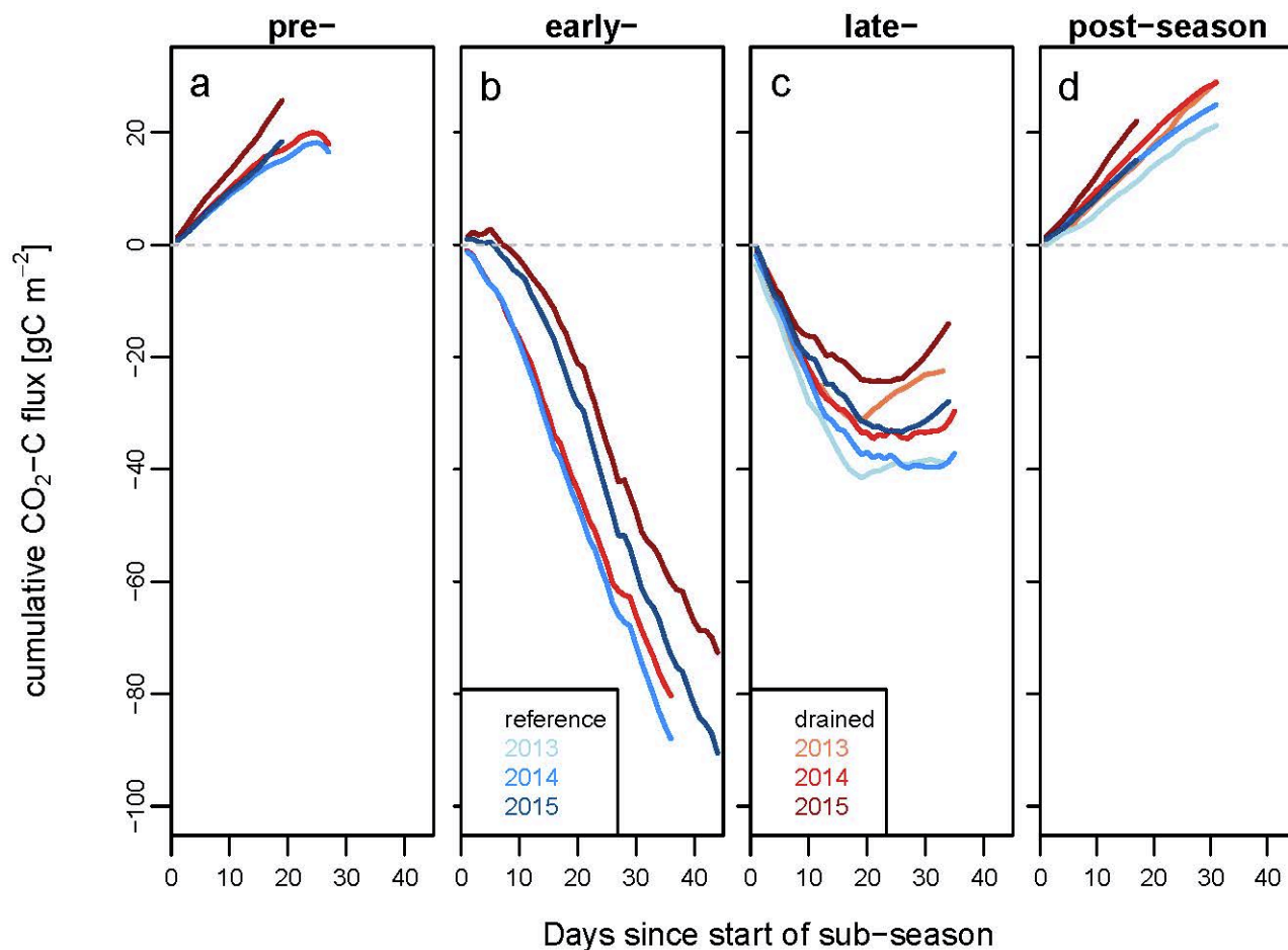
725 Figure 5: Cumulative CO 2 flux budgets for recent (2013–2015) eddy-covariance measurements for both sites (drained = red, reference = 730 blue). A grey line indicates the zero lines with a change from positive (i.e., release) and negative (i.e., uptake) fluxes. For these plots, timestamps have been normalized to account for interannual shifts in phenology. Time series were separated into the four different sub seasons (see Sect. 2.6) using individual key dates for each year. Time series were then plotted in separate panels, resetting the budgets to zero at the beginning of each sub-season. No measurements are available for the 2013 pre- and early-seasons, since measurements started mid-July 2013.
