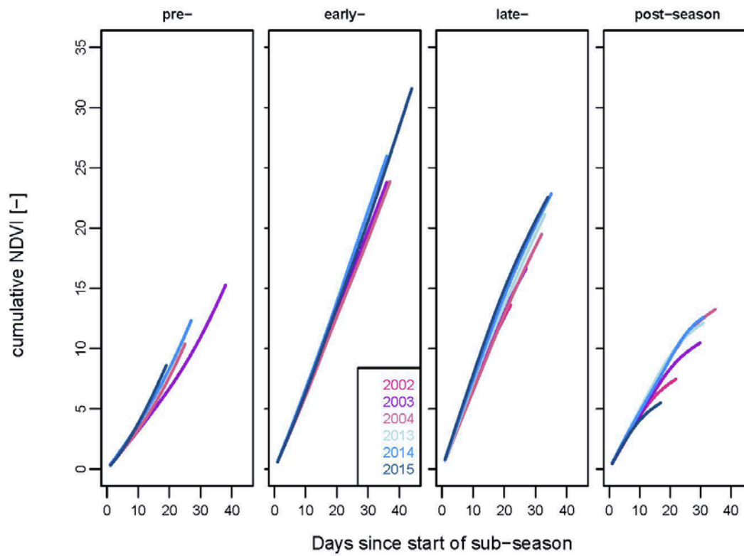
Figure B2: Sub-seasonal NDVI budgets for the reference area for the historic (2002–2004) and recent (2013–2015) datasets. Time axes 755 within this plotting scheme are identical to those used in Fig. 5.
