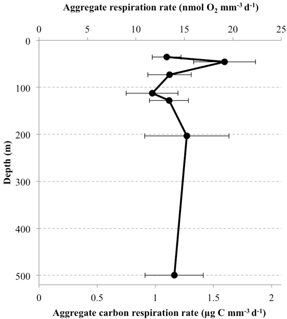
Figure 6: Respiration rates of phytodetrital aggregates with depth. Oxygen fluxes to aggregates (nmol O 2 mm -3 d -1 ) for natural aggregates collected at depth (black circles, solid black line) and roller tank formed aggregates (black triangle) . For reference aggregate respiration rates are also shown in terms of carbon per aggregate volume (µg C mm -3 d -1 ). Data are for experiments carried out at 10 °C. Error bars represent +/- 1 standard error.
