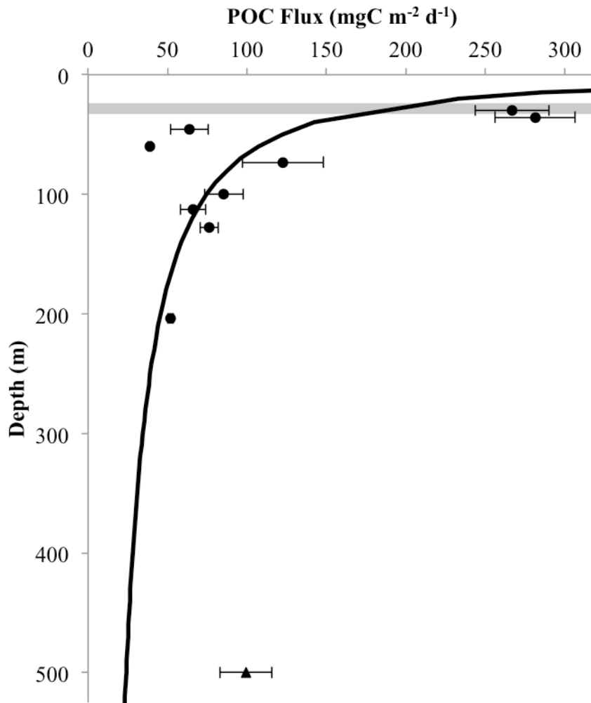
Figure 4: Flux of POC (mg C m -2 d -1 ) with depth at the PAP site. POC fluxes of fast-sinking fast-sinking particles measured in June 2015 at the PAP site via deployment of Marine Snow Catchers. Error bars relate to replicate filters per sample. A power-law curve was fitted to the data (black line), Y=194.9 \cdot (X/MLD)^{-0.71} ( R^2= 0.42 , p=0.060 , n=9 ), excluding the point at 500 m (triangle) which is likely due to non steady state conditions. The grey shaded area indicates the mixed layer depth over the study period.
