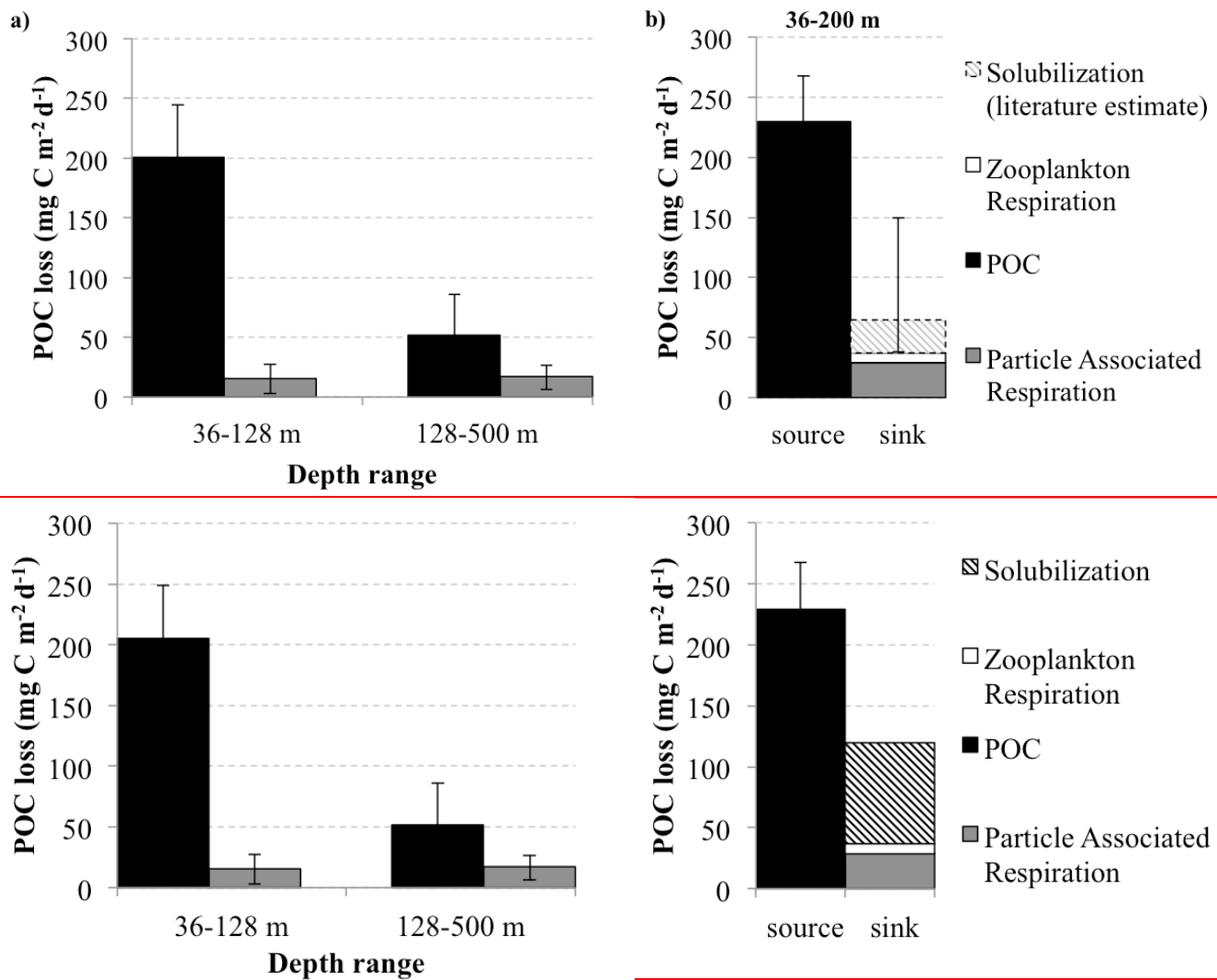
Figure 9: Balance of processes controlling fast-sinking POC flux attenuation. (a) Comparison of observed POC loss (black bars) and estimated POC loss based on particle associated microbial respiration only (grey bars) over two depth horizons (36-128 m, and 128-500 m). (b) Assessment of POC sources and sinks in the upper 200m. Additional estimated losses ('sinks') via solubilization of POC to DOC by particle associated microbes (calculated assuming respiration accounts for 25% of the total loss by particle associated microbes estimate based on respiration and solubilization the remaining 75%, see section 4.34), and zooplankton respiration (estimate based on zooplankton biomass and allometric equations) based on integrated (0-200 m) net data. Error bars show uncertainties from sensitivity analysis (see text for details). In figure (a) relate to the range in POC flux measured at each depth and the range in respiration rates calculated (see section 2.56). In figure (b) the errors from particle respiration measurements and zooplankton respiration estimates are summed. We include the possibility of solubilization as an additional sink term but cannot quantify errors as this term is poorly constrained. We do not display error bars on our assessments of POC sinks due to the potentially large and unconstrained errors on solubilization.
