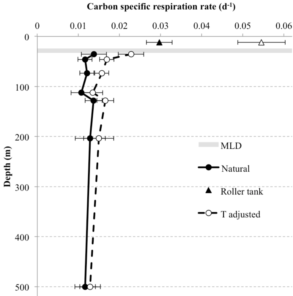
Figure 7: Carbon-specific respiration rates ( d^{-1} ) for natural aggregates collected at depth (black circles, solid line) and roller tank (triangles) formed aggregates; aggregates collected at depth. Rates adjusted to the in situ temperature (T) are shown by the dashed black line (open circles and open triangle for roller tank ). Grey shading shows the range in mixed layer depth over the study period, and error bars represent standard errors.
