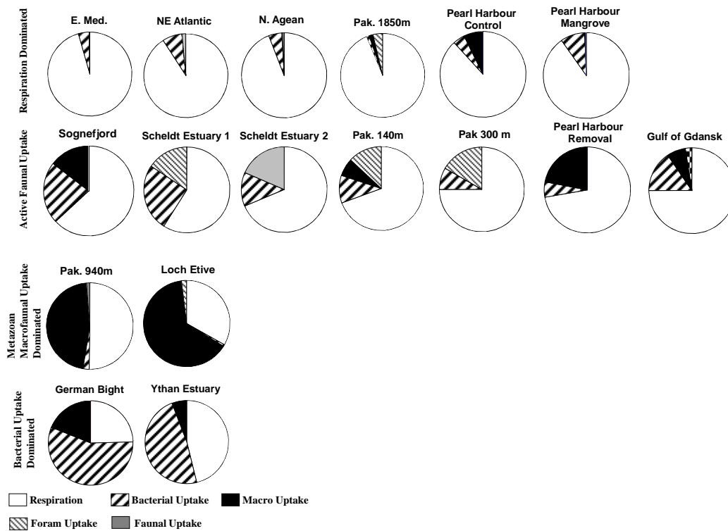
771 Figure 5. Biological C processing pattern categories adapted from Woulds et al. (2009), with the experiments 772 from this study and the new category ‘bacterial uptake dominated’ added. Data sources are as follows; Eastern 773 Mediterranean (E. Med.), NE Atlantic, North Aegean (N. Aegean) and Scheldt Estuary 2: Moodley et al. (2005); 774 ; Pakistan Margin (Pak. 140 m, 300 m, 940 m, 1850 m): Woulds et al. (2009); Sognefjord: Witte et al. (2003 a); 775 Scheldt Estuary 1: Moodley et al. (2000); Pearl Harbour: Sweetman et al. (2010); Gulf of Gdansk: Evrard et al. 776 (2012); German Bight: Buhring et al., (2006).
