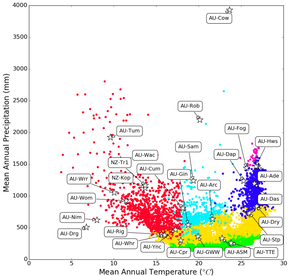
1050 Figure 2: OzFlux sites (white stars) across bioclimatic space with Fluxnet codes (Table 1). Mean annual temperature and mean annual precipitation are shown as the climate space using mean annual (1961-1990) gridded data (0.1 degree resolution) (Bureau-of-Meteorology, 2013). The colours represent the major modified Köppen climate classes (Stern and Dahni, 2013) as follows: 1) Equatorial (Pink), Tropical (Dark Blue), Sub-tropical (Light Blue), Desert (Green), Grassland (Yellow) and Temperate (Red).
